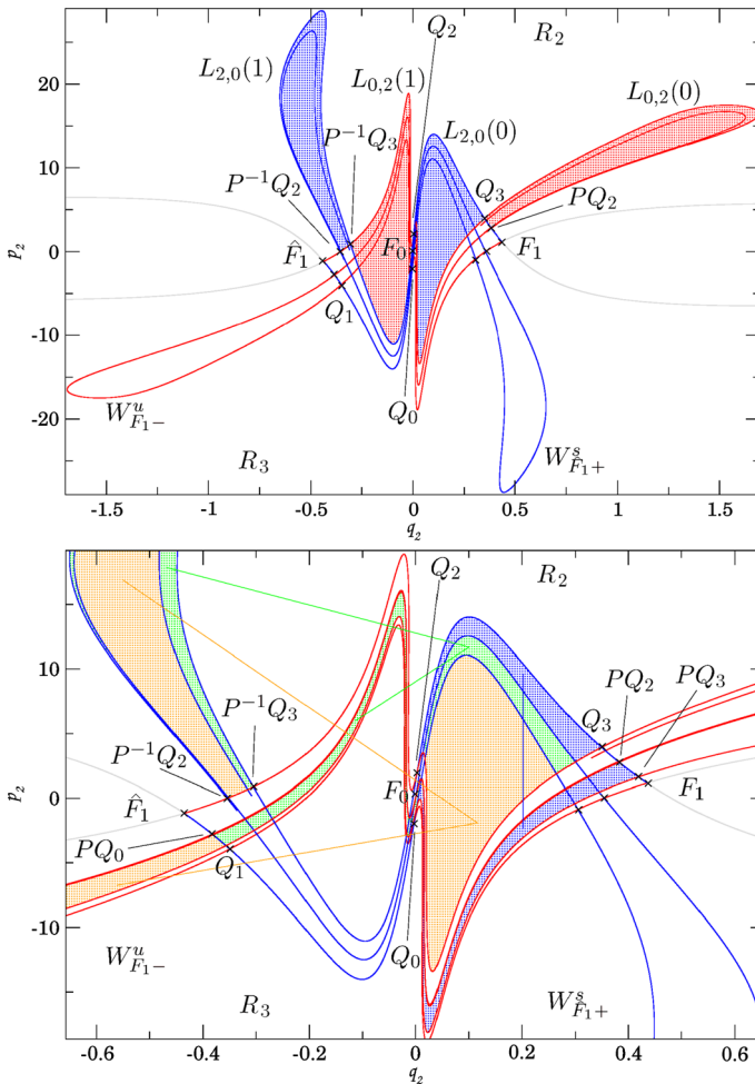
Fig. 24 The F_1-\widehat{F}_1 tangle at 0.02700 and an indication how certain parts of lobes are mapped in this tangle
