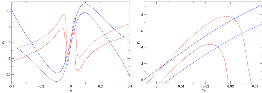
Fig. 27 The F_1 - \widehat{F}_1 tangle at 0.02550 and a detail of the diminished part of R_5 \setminus (R_6 \cup R_7)
