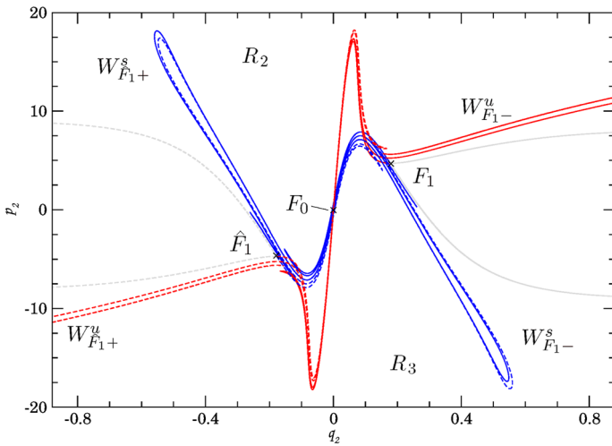
Fig. 17 The F_1-\widehat{F}_1 tangle at 0.02230, W_{F_1} are shown as solid lines, W_{\widehat{F}_1} as dashed
