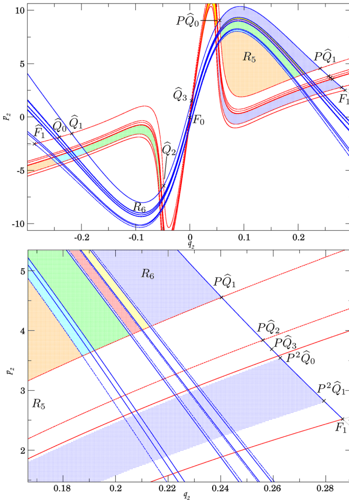
Fig. 28 Coloured sets in R_6 showing how part of the capture stripe is mapped at 0.02400. W_{F_1-} are drawn with solid lines, W_{\widehat{F}_1+} are dashed. CN_1 are shown in orange, CR_2 green and yellow, CN_2 red. Part of blue also belongs to CN_2 . Blue, yellow, red and green are separated by white stripes that are mapped to R_6 \cap R_7 (Color figure online)
