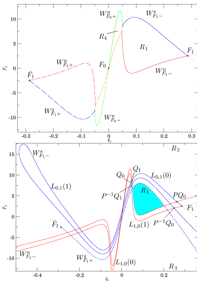
Fig. 22 Indication of boundaries of R_0 and R_4 (above) and the F_1 tangle at 0.02400 (below). The area in the F_1 tangle highlighted in cyan is the part of L_{0,1}(0) \cap L_{1,0}(1) that originates in products and is guided by W_{\hat{F}_1+}^s (dashed) into products (Color figure online)
