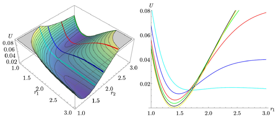
Fig. 2 The Porter–Karplus potential energy surface with contours and its cross sections for fixed values of r_2 = 1.70083 (cyan), 2 (blue), 2.5 (red), 3 (green), 4 (black), 50 (yellow) (Color figure online)
