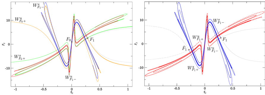
Fig. 23 Structure of the heteroclinic tangles at 0.02400. W_{F_0+} and W_{F_1-} making up the F_0 – F_1 tangle (left) and the F_1 – \widehat{F}_1 tangle (right). Unstable invariant manifolds are as indicated red and green, stable are blue and orange (Color figure online)
