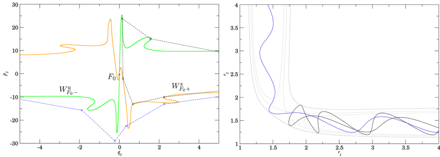
Fig. 10 Disjoint invariant manifolds of F_0 forming a barrier on \Sigma_0 at 0.01900 and examples of a nonreactive (black) and a reactive (blue) trajectory on \Sigma_0 and in configuration space (Color figure online)
