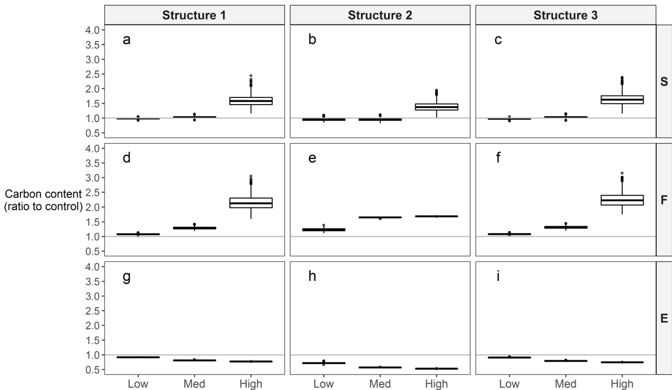
Fig. 3 Model simulation results showing the effect of different degrees of drought stress (low, medium and high) on soil carbon contents, expressed as the ratio of the carbon content in the drought stress simulation over the carbon content in the control simulation (no reduction of grazing rates).
