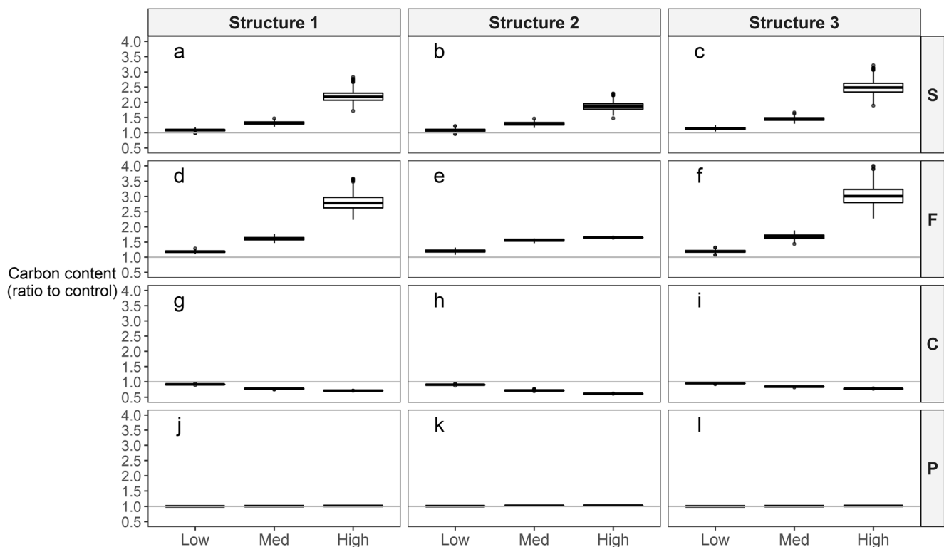
Fig. 4 Model simulation results of the more complex food web. Twelve different cases (a–l) are shown in separate panels: structures 1, 2 and 3 with the four different scenarios of stress sensitivities [same sensitivity (S); fungi more sensitive (F); consumers (enchytraeids, springtails and
