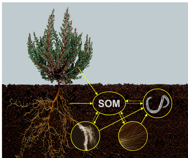
Fig. 1 Overview of carbon flow in the heathland soil food web whereby the considered uncertain links between groups are dashed. Circular illustrations (not to scale) from left to right: an ericoid mycorrhizal fungus (ERM) in symbiosis with its host plant, saprotrophic fungal (SF) mycelium and an enchytraeid worm. For the depiction of ERM and SF, figures were re-used with permission from Starrett et al. [17] and Crowther et al. [18], respectively
