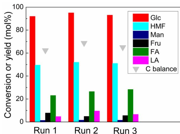
Fig. 14. Evaluation of the reusability of the combined \text{AlCl}_3/\text{HCl} catalyst in the glucose conversion in the slug flow capillary microreactor at the optimized reaction conditions using 0.1 M glucose solution as the feedstock (as those shown in Fig. 2).
