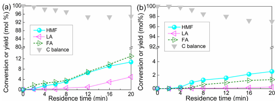
Fig. 4. Results of experiments with HMF as the substrate in a biphasic system in the slug flow capillary microreactor with (a) \text{AlCl}_3 and (b) HCl as catalyst. Other reaction conditions: 160 °C, 0.1 M reactant solution, microreactor length of 4.5 m, 40 mM \text{AlCl}_3 or 0.39 mM HCl (both yielding pH = 3.4 at 20 °C), 4:1 organic to aqueous inlet flow ratio.
