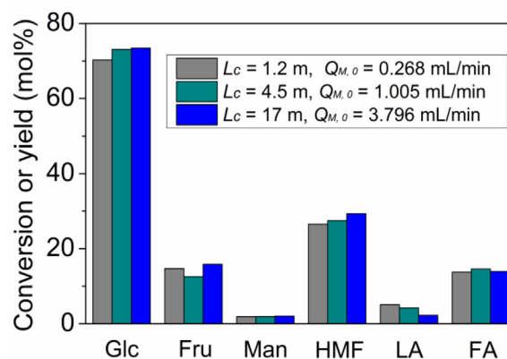
Fig. 13. Glucose conversion and product yields in the slug flow capillary microreactor of different lengths. Reaction conditions: 0.1 M glucose, 160 °C, 40 mM AlCl 3 and 40 mM HCl (pH = 1.5 measured at ca. 20 °C), 8 min residence time, 4:1 organic to aqueous inlet flow rate ratio. In the legend, Q_{M,0} represents the total volumetric flow rate of the two-phase mixture at the microreactor inlet.
