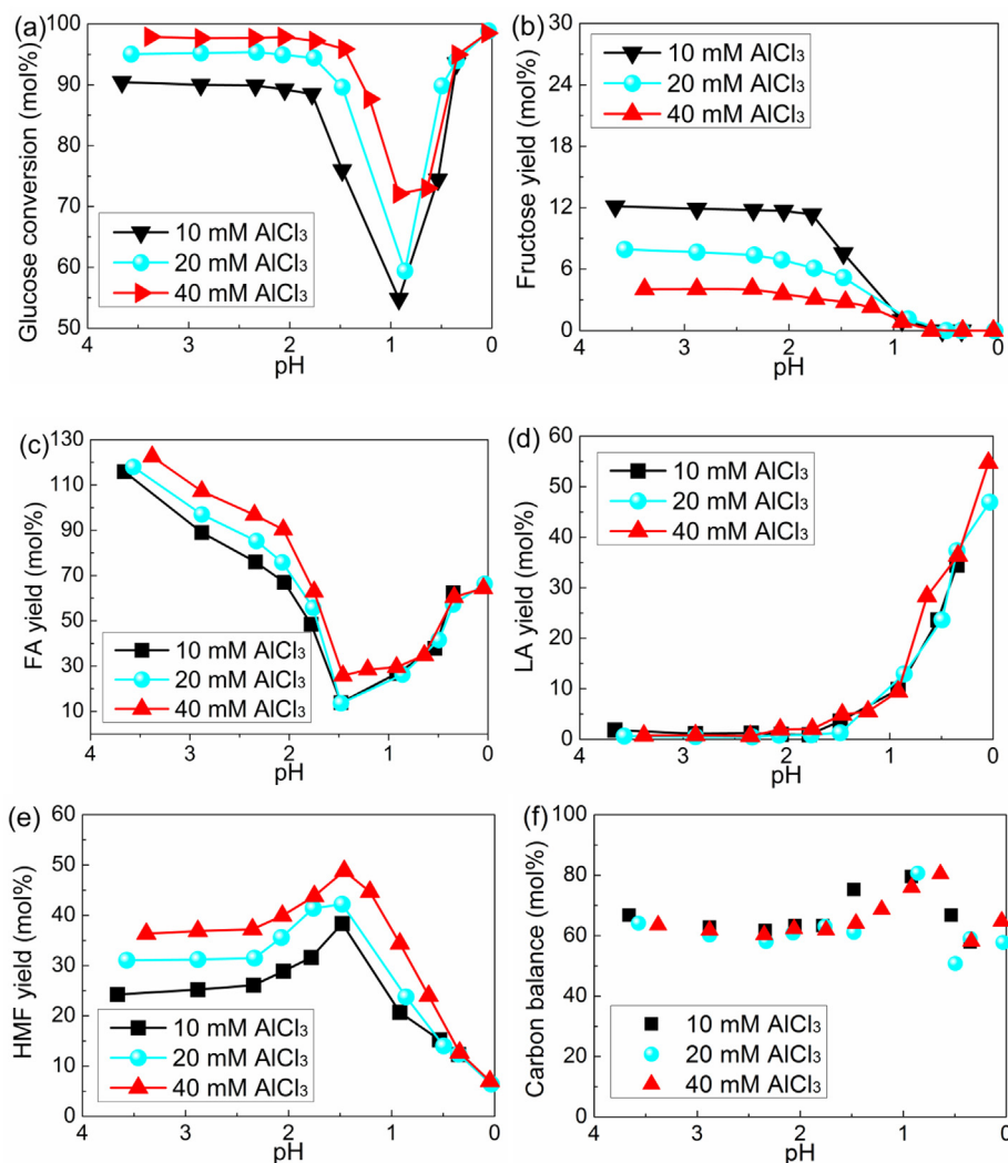
Fig. 8. Effect of Brønsted acidity on the glucose conversion reaction performance in the slug flow capillary microreactor using \text{AlCl}_3 and HCl as catalyst. (a) glucose conversion; (b) fructose yield; (c) FA yield; (d) LA yield; (e) HMF yield; (f) carbon balance. Other reaction conditions: 0.1 M glucose, 160^\circ\text{C} , microreactor length of 4.5 m, residence time at 16 min, 4:1 organic to aqueous inlet flow ratio, pH values were adjusted by the addition of HCl in the aqueous phase and reported according to the measurement at ca. 20^\circ\text{C} .
