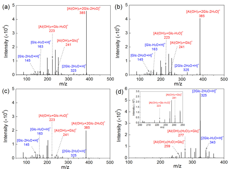
Fig. 10. ESI-MS spectra of the fresh aqueous 0.1 M glucose solution containing (a) 40 mM \text{AlCl}_3 (pH = 3.38); (b) 40 mM \text{AlCl}_3 and 40 mM HCl (pH = 1.5); (c) 40 mM \text{AlCl}_3 and 640 mM HCl (pH = 0.34); and (d) MS/MS spectra of the selected [\text{Al}(\text{OH})_2 + 2\text{Glc}]^+ species of sample (b) with m/z of 385. Inset in (d) shows a magnified view of m/z region at 200–250.
