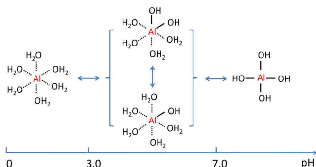
Fig. 9. Schematic representation of Al (III) cations in water under different Brønsted acidities.
