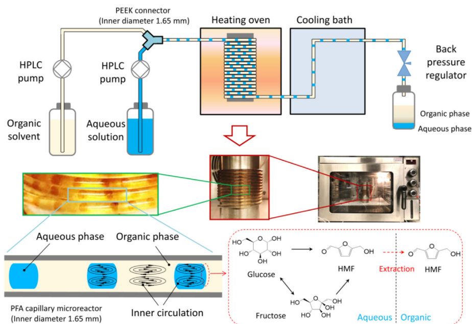
Fig. 1. Schematic diagram of the slug flow capillary microreactor system for continuous HMF synthesis from glucose. The inner circulation in droplets and slugs promoted mixing/reaction in the aqueous phase and enhanced in-situ extraction of HMF to the organic phase.
