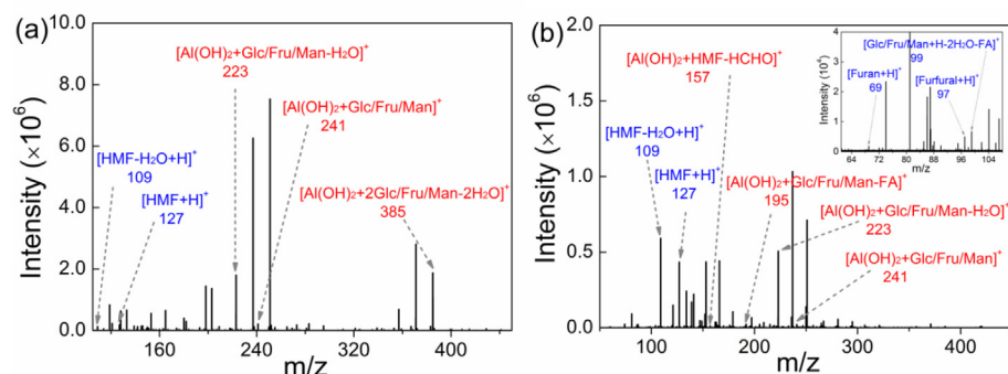
Fig. 11. ESI-MS spectra of the aqueous product sample collected after the reaction of 0.1 M glucose solution containing 40 mM \text{AlCl}_3 and 40 mM HCl ( \text{pH} = 1.5 measured at ca. 20^\circ\text{C} ) in the microreactor for a residence time of (a) 4 min and (b) 16 min. Inset in (b) shows a magnified view of m/z region at 80–108. Other reaction conditions: 160^\circ\text{C} , microreactor length of 4.5 m, 4:1 organic to aqueous inlet flow ratio.
