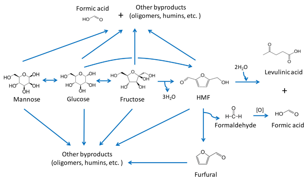
Fig. 3. Proposed reaction network for the glucose conversion to HMF.
