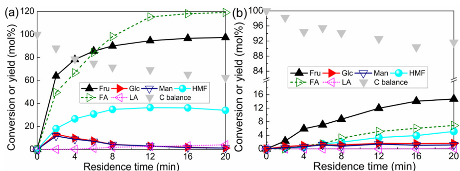
Fig. 5. Results of experiments with fructose as the substrate in a biphasic system in the slug flow capillary microreactor with (a) \text{AlCl}_3 and (b) \text{HCl} as catalyst. Other reaction conditions are the same as those specified in Fig. 4.
