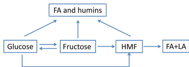
Fig. 7. Simplified view of the main reaction routes during HMF synthesis from glucose (based on the details depicted in Fig. 3).
