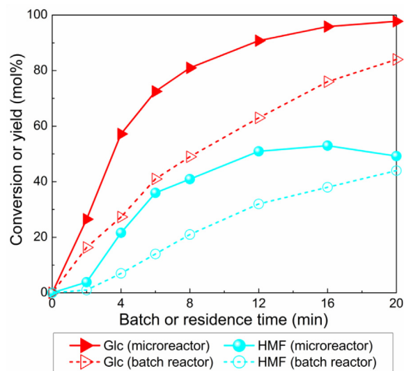
Fig. 12. Glucose conversion and HMF yield as a function of the residence time in the microreactor and the batch time in the batch reactor in a biphasic system at optimized conditions. Reaction conditions: 0.1 M glucose, 160^\circ\text{C} , 40 mM \text{AlCl}_3 and 40 mM HCl ( \text{pH} = 1.5 measured at ca. 20^\circ\text{C} ), organic to aqueous inlet flow ratio or initial volume ratio at 4:1.
