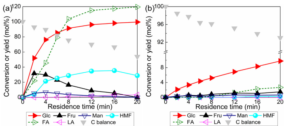
Fig. 6. Results of experiments with glucose as the substrate in a biphasic system in the slug flow capillary microreactor with (a) \text{AlCl}_3 and (b) \text{HCl} as catalyst. Other reaction conditions are the same as those specified in Fig. 4.
