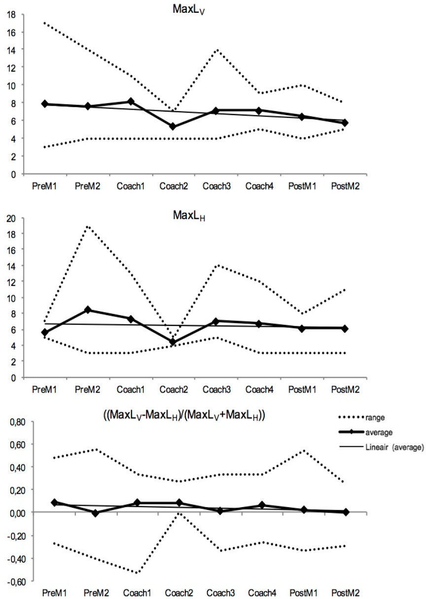
Fig. 7. Average maximum line (MaxLv, MaxLH and ((\text{MaxLv}-\text{MaxLH})/(\text{MaxLv}+\text{MaxLH})) ) over eight science lessons. Solid line indicates average of teachers and dotted line indicates the range (minimum and maximum values).
