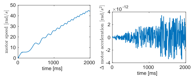
Figure 2: SimScape simulation
