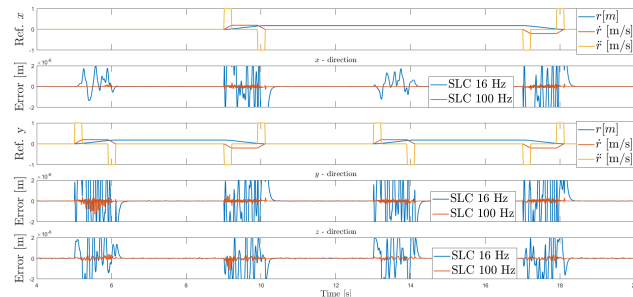
Figure 3: x , y reference profiles and position errors in x , y , z axes for the initial 16Hz and the 100Hz , SLC controller.
