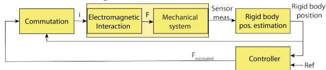
Figure 2: Block diagram of the NAPAS experimental setup
