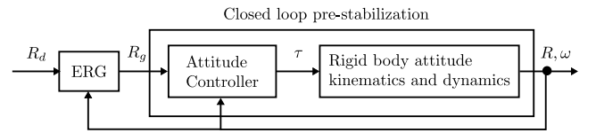
Figure 2: Control scheme
