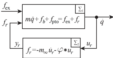
Figure 1: Single floater interconnection with the radiation force.
