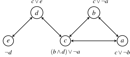
Figure 1. Symmetric ADF which is neither semi-coherent, weakly coherent nor relatively grounded.
