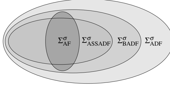
Figure 3. Expressiveness of subclasses of ADFs for \sigma \in \{adm, prf, com\}
