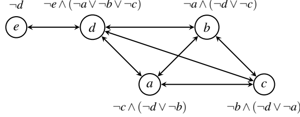
Figure 2. ASSADF without supporting links being not semi-coherent.
