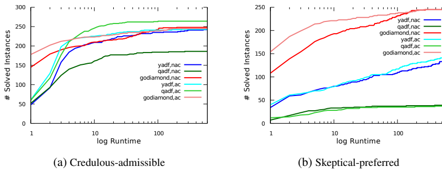
Figure 4. Plot of running time (in seconds) vs. number of instances solved (out of all benchmarks) for all ADF solvers. “ac” stands for “acyclic”, “nac” for “non-acyclic”.
