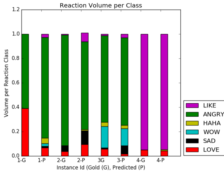
Figure 2 Plot of the reactions’ volume per reaction class of the examples in Table 8. Each gold instance (G) is paired with the predicted one (P). Volumes are normalized between 0 and 1.
