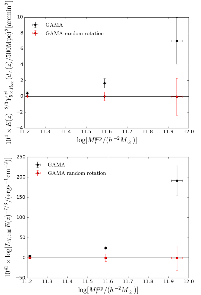
Figure D1. Top panel: The stacked Y_{5 \times R_{500}} - M_{*,\text{GFP}} relation for the GAMA galaxy groups (black) and mean of 1000 realisations of the GAMA groups randomly rotated along their galactic latitude (red). Bottom panel: Similar comparison, but for the X-ray luminosity. In both cases we see that the signal vanishes when we randomize the positions of the groups.
