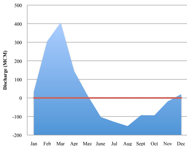
Figure 11: Monthly stream flow surplus and deficit for Santa River at the La Balsa station in 2007; Source: Autoridad Local del Agua
