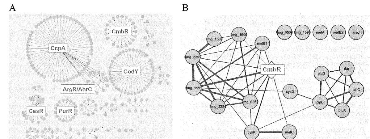
Figure 2. L. lactis regulons and CmbR regulon cliques Cytoscape Network of known regulons in L. lactis MG1363. A) The known regulons in L. lactis ; diamond shapes are TFs and circle shapes are genes. An arrow indicates activation and a blunt-end line shows repression of the gene by the TF. B) All CmbR regulon members connected via Pearson correlations derived from time-series transcriptomics data. The thickness of the lines (edges) corresponds to the strength of co-expression.
