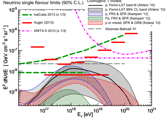
Figure 6: Upper limits to the diffuse flux of UHE neutrinos at 90% C.L. in integrated (horizontal lines) and differential form. Limits described in this work (red lines) are compared with cosmogenic neutrino models [16, 17, 18], the Waxman-Bahcall bound [19], and limits from IceCube [20] and ANITA [21]. All neutrino limits and fluxes are converted to single-flavour.
