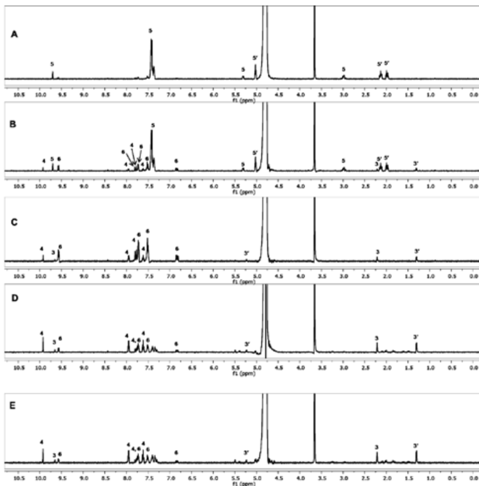
Supplementary Figure 5 – Stack plot of ^1\text{H} NMR spectra recorded after 18 h of incubation of 5 with A) no enzyme; B) wild-type 4-OT; C) 4-OT F50V; D) 4-OT M45T/F50A; and E) 4-OT H6F/M45T/F50A. Signals corresponding to 3 and its hydrated ( 3' ), 4, 5 and its hydrate ( 5' ), and 6 are marked.
