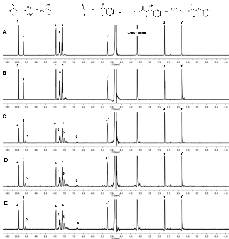
Supplementary Figure 3 – Stack plot of ^1\text{H} NMR spectra recorded after 1 d of incubation of 3 and 4 with A) no enzyme; B) wild-type 4-OT; C) 4-OT F50V; D) 4-OT M45T/F50A; and E) 4-OT H6F/M45T/F50A. Signals corresponding to 3 and its hydrate (3'), 4 and 6 are marked.
