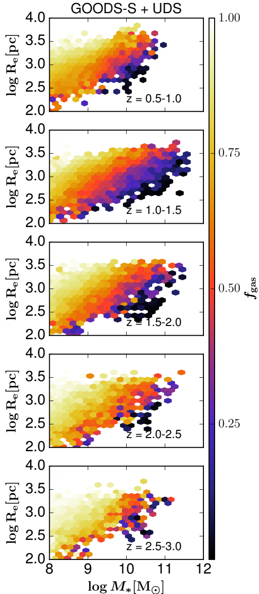
Figure 14. Galaxy scale radius as a function of stellar mass for different redshift bins. The colour map gives the cold gas fraction.
