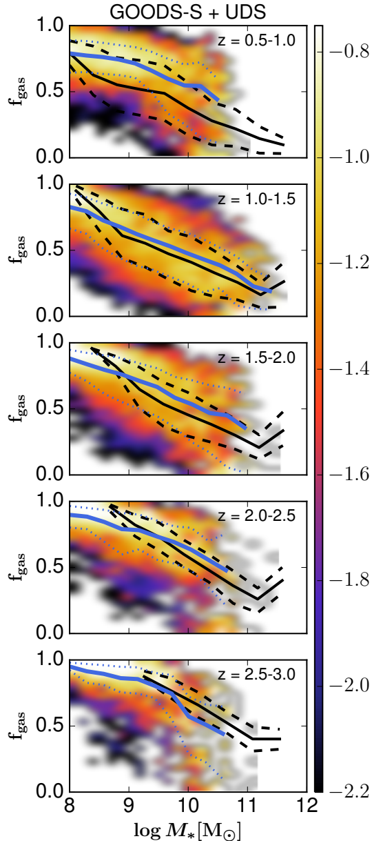
Figure 7. Cold gas fraction of galaxies ( f_{\text{gas}} \equiv \frac{M_{\text{H2+HI}}}{M_{\text{H2+HI}+M_*} ) as a function of stellar mass and redshift. The shaded regions show the log of the conditional probability distribution function P(f_{\text{gas}}|M_*) , and the blue solid and dotted lines show the median fit and one \sigma deviation. The black solid and dashed lines show the mean fit and one \sigma deviation to the predictions of Popping, Somerville & Trager (2014).
