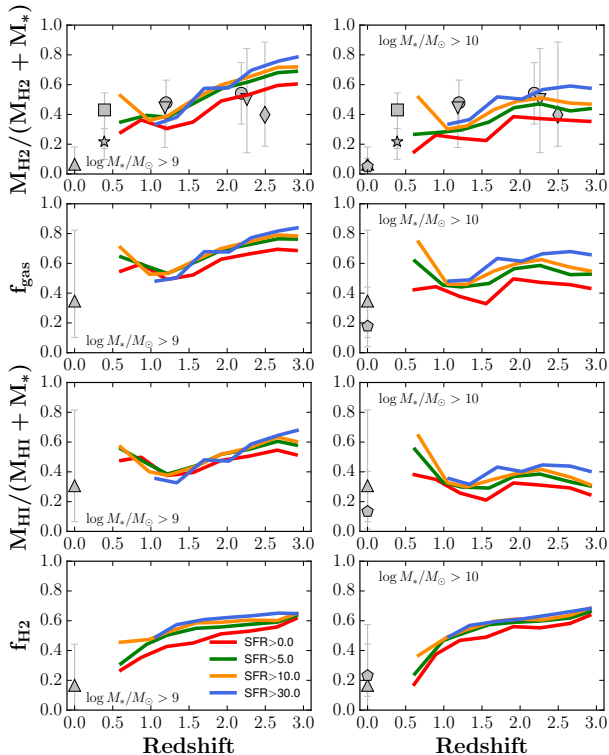
Figure 18. Redshift evolution of the relative H 2 content \frac{M_{\text{H}_2}}{M_{\text{H}_2} + M_*} (top row), gas fraction (second row), relative HI content (third row), and molecular hydrogen fraction (bottom row) for galaxies with stellar masses in the range M_* > 10^9 M_\odot (left panels), M_* > 10^{10} M_\odot (right panels), and SFR larger than 0 (red), 5 (green), 10 (orange), and 30 (blue) M_\odot \text{yr}^{-1} . Different markers represent the following datasets: upwards pointing triangles : galaxies from the THINGS survey (Leroy et al. 2008) at z = 0.0 , pentagons : galaxies from the COLD GASS survey (Saintonge et al. 2011) at z = 0.0 , squares : galaxies from Bauermeister et al. (2013) at z \sim 0.4 , stars : galaxies from Geach et al. (2011) at z \sim 0.4 , circles : galaxies from the PHIBBS survey (Tacconi et al. 2013) at z \sim 1.2 and z \sim 2.2 , downwards pointing triangles : galaxies at z \sim 1.2 and z \sim 2.2 from Tacconi et al. (2010), diamonds : galaxies at z \sim 2.2 from (Saintonge et al. 2013). Error bars show the 80 percent confidence interval for each observational sample at the given redshift bin.
