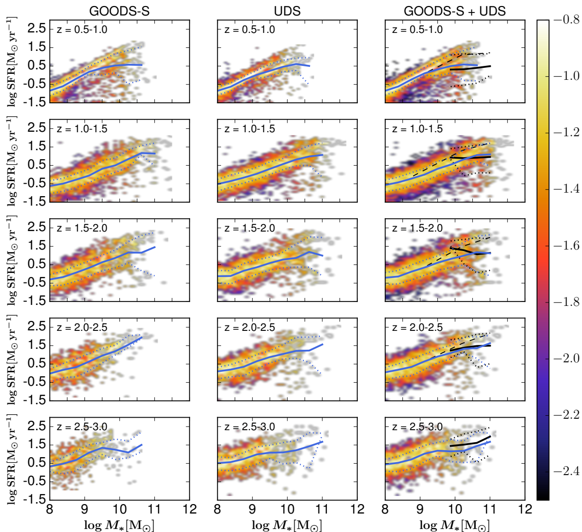
Figure 3. Galaxy SFR as a function of stellar mass in different redshift bins. The shaded regions show the log of the conditional probability distribution P(\text{SFR}|M_*) , which represents the probability distribution of SFRs for fixed stellar masses, and the blue solid and dotted lines show the median fit and 2\sigma deviation. The left column shows results for the GOODS-S sample, the middle column for the UDS sample, and the right column for the combined GOODS-S and UDS sample. The black line marks the mean trend of the UV + IR based SFRs presented in Barro et al. (2014) in the GOODS-S and UDS fields. The black dashed line mark the double-power-law fit to the relation between stellar mass and SFR presented in Whitaker et al. (2014).
