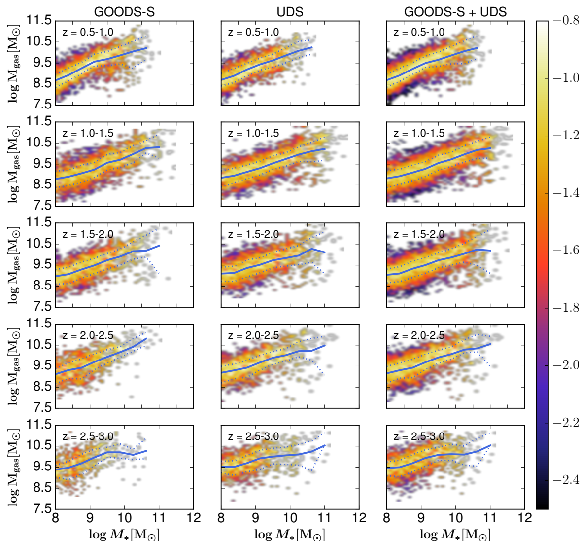
Figure 4. Total cold gas mass of galaxies as a function of their stellar mass in different redshift bins. The shaded regions show the log of the conditional probability distribution P(M_{\text{gas}}|M_*) , and the blue solid and dotted lines show the median fit and one \sigma deviation. Columns are as described in the caption of Figure 3.
