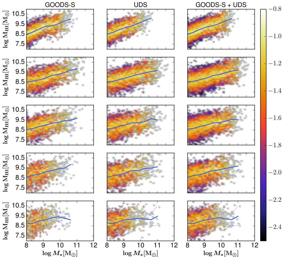
Figure 6. The HI mass of galaxies as a function of their stellar mass in different redshift bins. The shaded regions show the log of the conditional probability distribution P(M_{\text{HI}}|M_*) , and the blue solid and dotted lines show the median fit and one \sigma deviation. Columns are as described in the caption of Figure 3.
