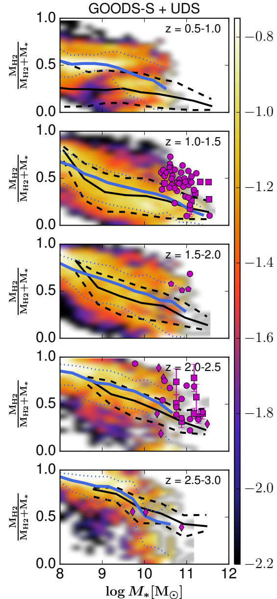
Figure 8. Relative molecular content as a function of stellar mass for different redshift bins. The shaded region shows the log of the conditional probability distribution function P(\frac{M_{\text{H2}}}{M_{\text{H2}+M_*}}|M_*) , and the blue solid and dotted lines show the median fit and one \sigma deviation. The black solid and dashed lines show the mean fit and one \sigma deviation to the predictions of Popping, Somerville & Trager (2014). Purple pentagons, circles, squares and diamonds are literature values from Daddi et al. (2010), Tacconi et al. (2010), Tacconi et al. (2013), and Saintonge et al. (2013), respectively.
