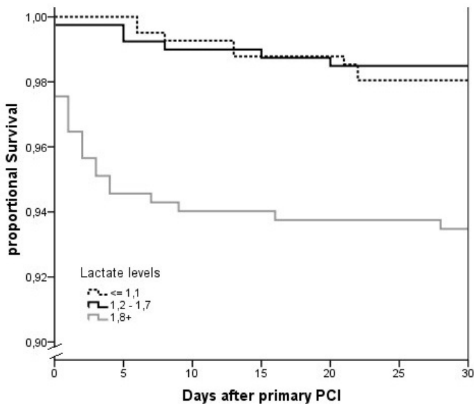
Figure 2 Kaplan-Meier curve displaying 30-day proportional survival after primary PCI.
