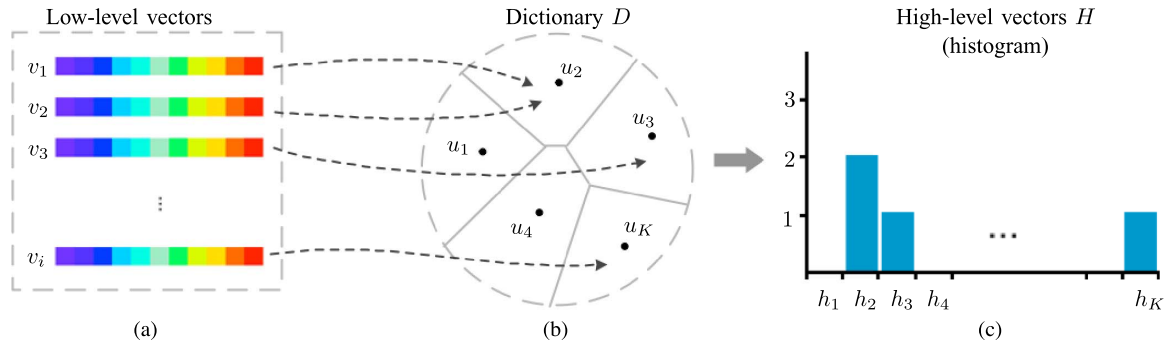
Fig. 1. Construction of the high-level representation. For each vector v_i the nearest audio word u_j in the dictionary is determined (b). Then, the occurrence counts of the single audio words are stored in a histogram, whose bins are h_j (j = 1, \dots, K) that constitutes the high-level vector (c). In the example, vectors v_1 and v_2 have u_2 as the nearest audio word in the dictionary. Thus, the second bin of the histogram has a value equal to 2. In the same way, audio word u_3 has only one close vector, resulting in a value equal to 1 for the third bin of the histogram. Audio words u_1 and u_4 , instead, have no occurrences.
