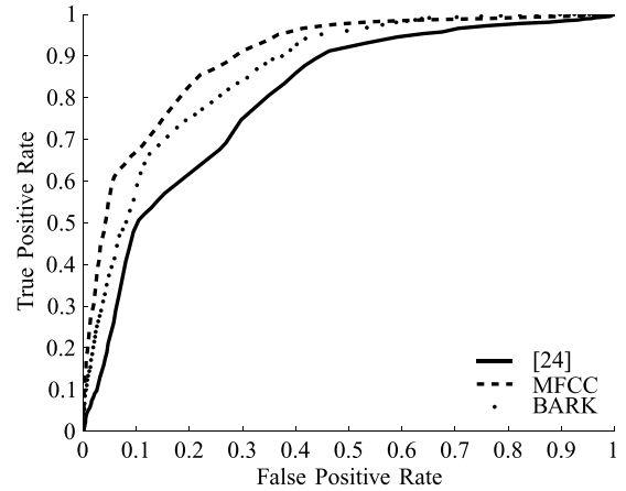
Fig. 6. ROC curves of the proposed system configured with the three considered sets of features.
