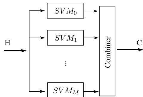
Fig. 2. Architecture of the classifier. The scores of the SVM classifiers are combined in order to determine the final class to be assigned to the input vector H .
