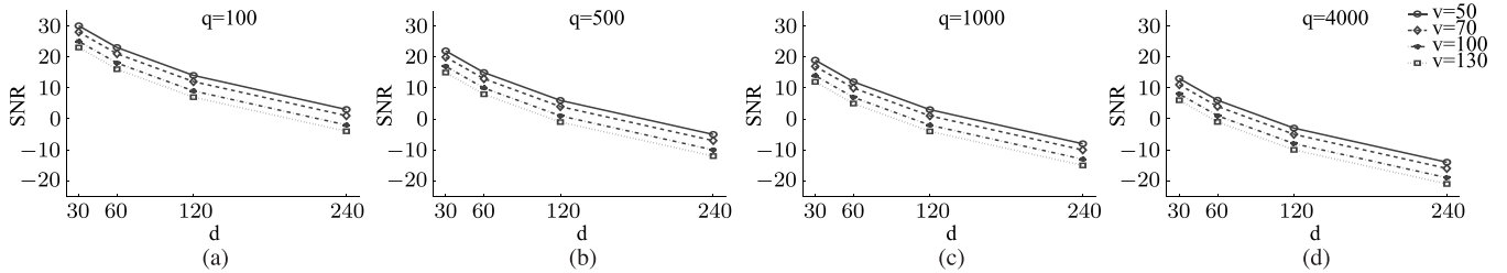
Fig. 4. Variation of the value of SNR (expressed in dB) with respect to the distance d (expressed in meters) the average speed v (expressed in km/h) and the traffic flow q (expressed in vehicles/h).
