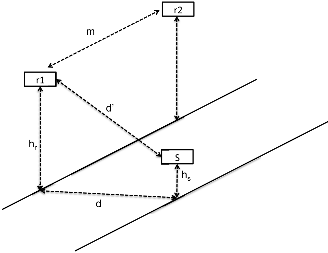
Fig. 3. A sketch of the deployment of the proposed system: a set R of microphones is located at a distance of m meters far from each other and at a height h_r . An event of interest can be recognized at a maximum distance of d meters from the closest microphone.
