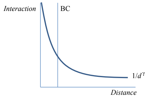
FIGURE 2: Distance Decay.
