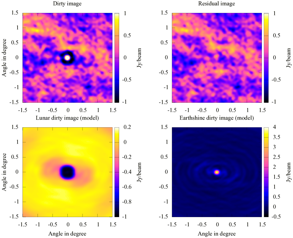
Figure 5.7: Plot demonstrating the mitigation of reflected RFI (Earthshine) in lunar images. Top left panel shows a dirty image of the Moon at 68 MHz contaminated by Earthshine. Bottom-left panel shows the reconstructed dirty image of the Moon with Earthshine removed. Bottom-right panel shows the reconstructed dirty image of Earthshine only, and top-right panel shows the residuals of model fitting.
