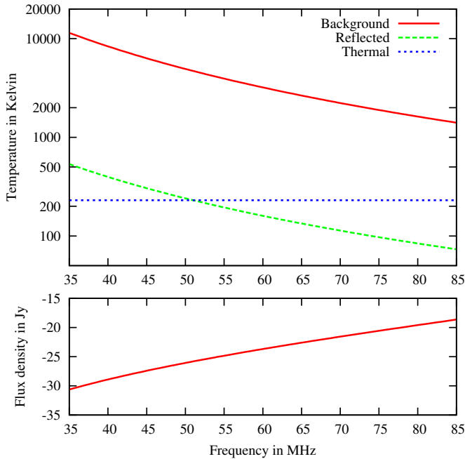
Figure 5.2: Plot showing the expected temperature of occulted Galactic synchrotron emission, reflected Galactic emission, and lunar thermal emission as a function of frequency (top panel), and also the resulting flux density of the Moon as measured by an interferometer (bottom panel).
