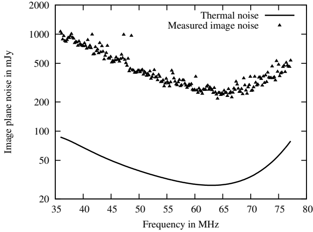
Figure 5.6: Plot showing noise estimated in the lunar images. The thermal noise was estimated by differencing visibilities between frequency channels separated by about 40 kHz. The measured image noise is shown for naturally weighted images ( 20\lambda - 500\lambda baselines) made over a bandwidth of about 195 kHz with a 7 hour synthesis.
