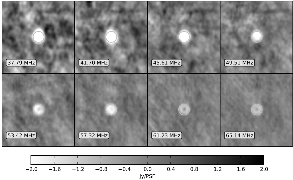
Figure 5.5: Synthesis images of the Moon at 8 different frequencies: 0.5 deg wide gray circles are drawn centered on the expected position of the Moon. Each image is made over a bandwidth of 3.9 MHz (20 sub-bands) for 7 hours of synthesis. The lunar flux increases towards zero with increasing frequency as the contrast between the Galactic background and lunar thermal emission is decreasing (as expected).
