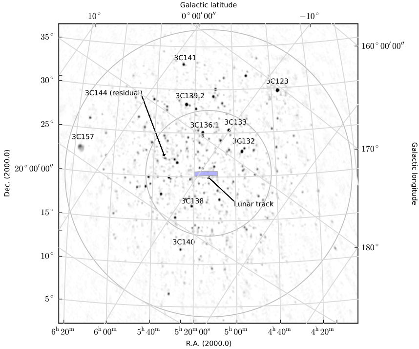
Figure 5.4: Continuum image of the lunar field between 36 and 44 MHz (natural weights) with no primary-beam correction applied. The point spread function is about 12 arcmin wide. Prominent 3C source names have been placed right above the respective sources. 3C144 (Crab nebula) has been subtracted in this image. The gray circles approximately trace the first null of the primary beam at 35 (outer) and 80 MHz (inner). The shaded rectangular patch shows the trajectory of the Moon during the 7 hr synthesis. We have not fringe-stopped on the Moon (moving source) in producing this image, and hence the Moon is not visible due to the ensuing decorrelation.
