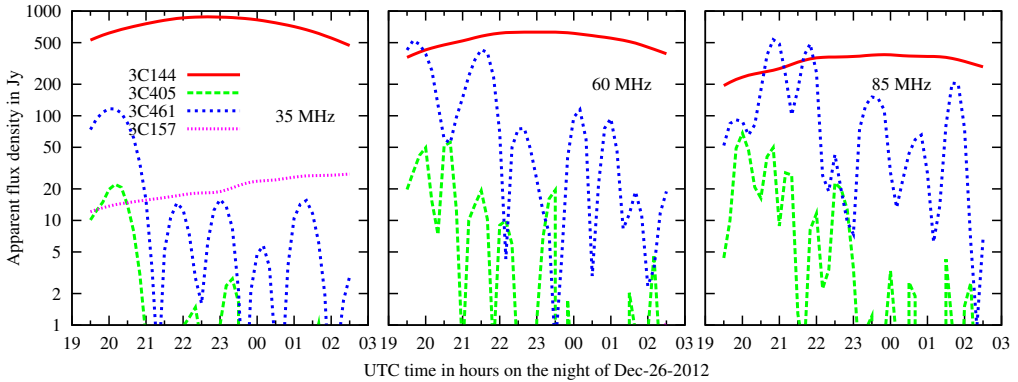
Figure 5.3: Plot showing the simulated apparent flux (primary-beam attenuated) of sources which dominate the flux budget in the lunar field for three different frequencies: 35 MHz, 60 MHz, and 85 MHz. The modulations in time are due to the sources moving through the sidelobes of the primary (station) beam during the synthesis.
