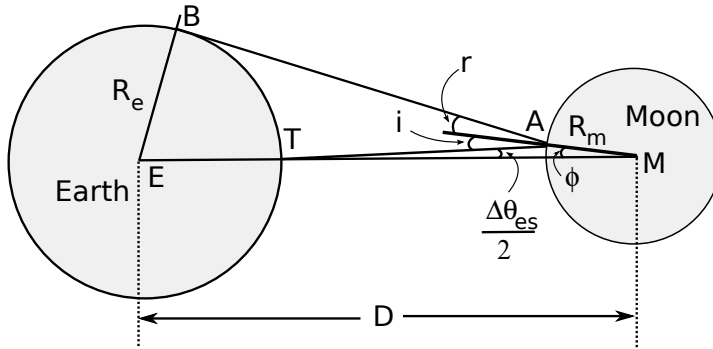
Figure 5.11: Not-to-scale schematic of the Earth-Moon geometry used in the calculation of the angular size of reflected Earthshine
