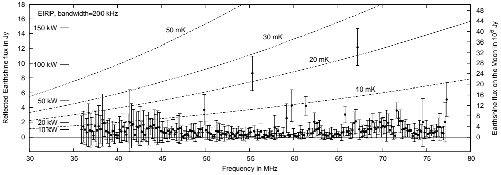
Figure 5.9: Plot showing the reflected Earthshine (left-hand y axis) and Earthshine as seen by an observer on the Moon (right-hand y axis). At each frequency channel (195 kHz wide), we measure 7 values of Earthshine each from a one hour synthesis images (7 hours in total). Plotted are the mean and standard deviation of the 7 Earthshine values at each frequency channel. Also shown are 5 EIRP levels of the Earth in a 195 kHz bandwidth. The dotted lines denote the flux level in a single dipole for different brightness temperatures of 10, 20, 30, and 50 mK.
