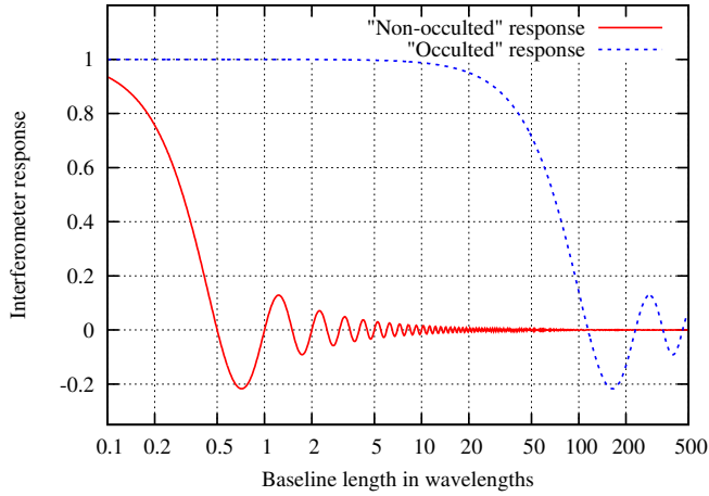
Figure 5.1: Normalized response of an interferometer to lunar occultation as a function of baseline length: the blue broken line shows the ‘occulted’ component (Equation 5.7) and the solid red line shows the ‘non-occulted’ component (Equation 5.6). The solid red line is also the interferometer response in the absence of occultation.
