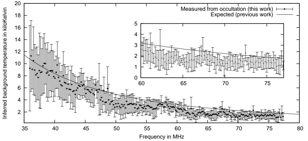
Figure 5.8: Plot showing the inferred background temperature occulted by the Moon. At each channel, we estimate 7 background temperature values using 7 one-hour synthesis images of the Moon. Plotted are the mean and standard deviation of the 7 temperatures measured in each channel.
