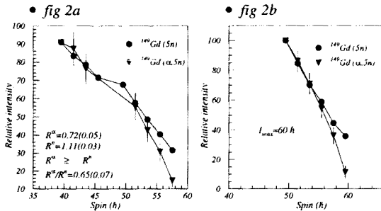
Fig. 2. Feeding of the superdeformed yrast band of ^{149}\text{Gd} . In Fig. 2a R represents the intensity of the bands, I_{\max} is the highest spin observed in \alpha n channel.
