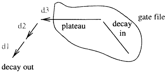
Fig. 2. Schematic view of the intensity pattern of a SD band. One gate file involves the plateau (minus the last transition) and the decay in, the other file contains one gate on the deexcitation line or on the last transition of the plateau.
