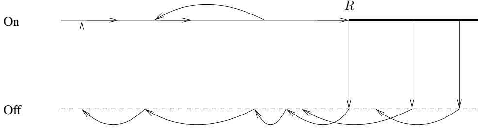
Figure 1: The state space of the inventory process. The thick bar on the on-line represents the subset at which the policy \pi_R decides to switch production off. The off-line is dashed to indicate that the inventory does not decrease continuously, but in jumps.
