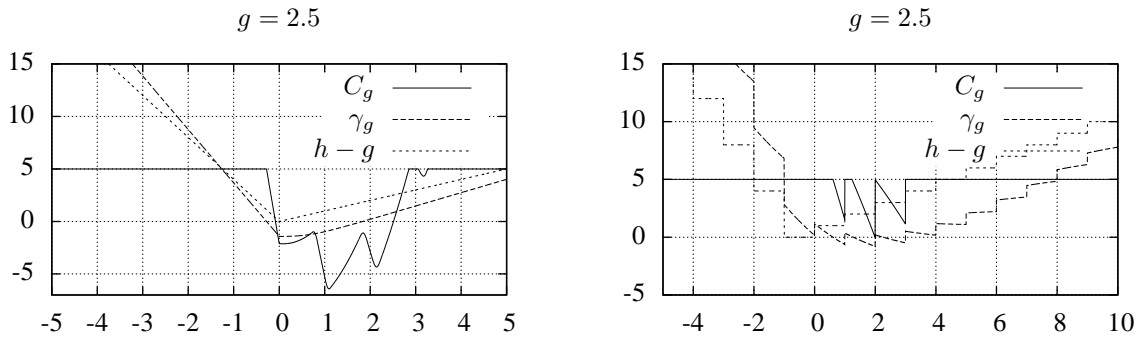
Figure 3: The left panel shows C_g when the demand is deterministic D \equiv 1 . The appearance of the small dent at the right of S implies that the optimal policy is not monotone. The right panel shows C_g for quasi-convex holding costs. The fact that the value function hits K between s and S implies that the optimal policy is not (s, S) .
