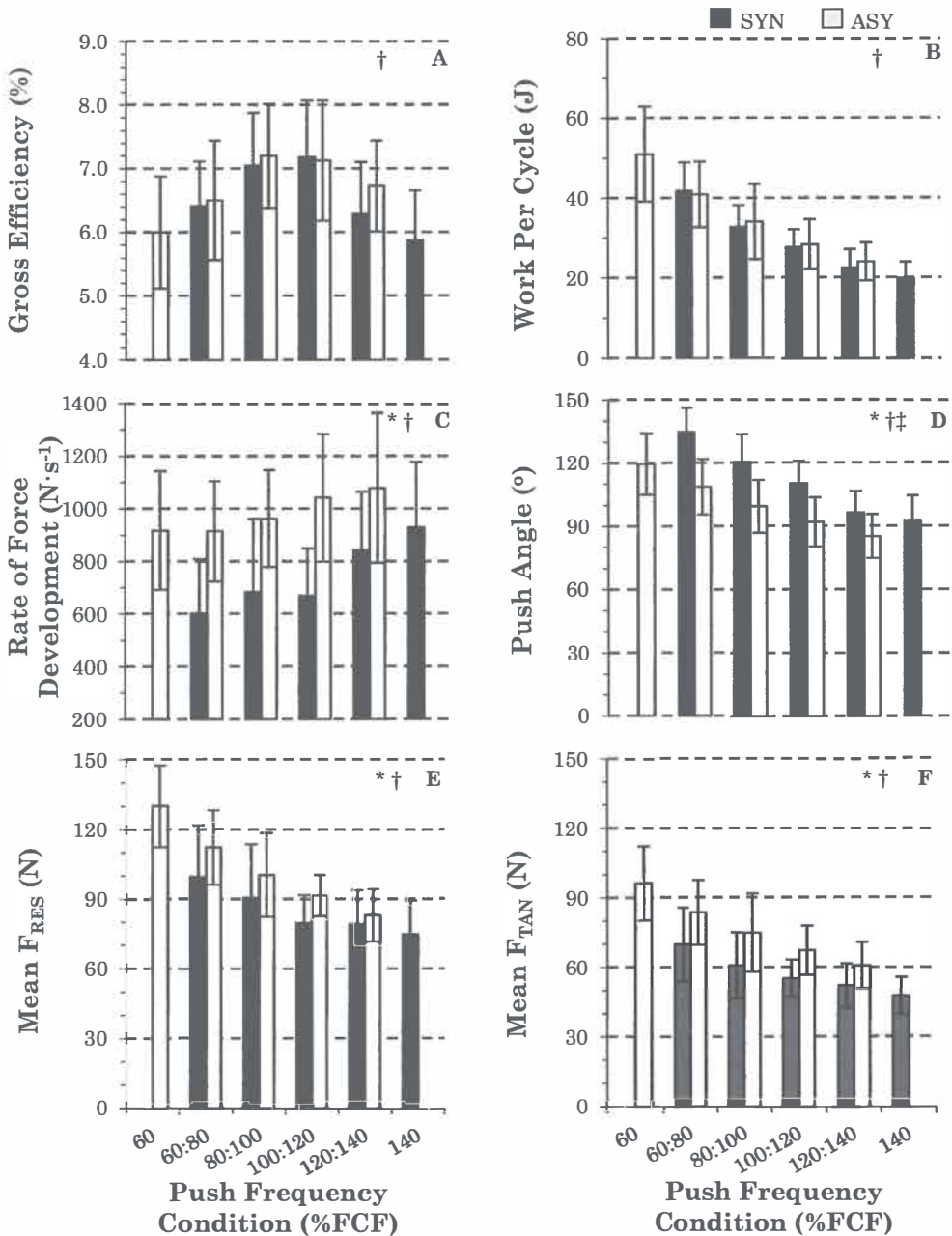
Fig 7.3: Matched Push Frequencies: Mean values \pm SD for selected force parameters, timing and efficiency in synchronous (SYN) and asynchronous (ASY) hand-rim propulsion across matched push frequencies. (A) gross efficiency, (B) work per cycle, (C) rate of force development, (D) push angle, (E) mean resultant force and (F) mean tangential force. * Significant main effect mode (ASY vs. SYN). † Significant main effect frequency. ‡ Significant main effect mode*frequency ( P \leq 0.05 ).
