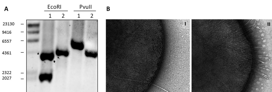
Figure 4. Southern blot analysis of wild-type Pil + S. acidocaldarius MR31 (1) and Pil - (2) strain (A) to confirm knockout of upsEF genes. Expected fragment sizes for WT MR31: 3906 bp and 2128 bp for EcoRI and 6785 bp for PvuII (1). Expected fragment sizes for knockout of upsEF : 4593 bp for EcoRI and 5344 for PvuII (2). Electron micrographs of Pil - strain with UV (BI) and Pil + strain with UV (BII). Only flagella like structures can be observed on the cell surface of UV-treated Pil - cells and no short straight UV pili (B). Scale bar is 0.2 \mu m in length.
