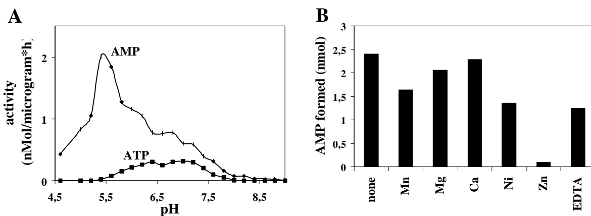
Fig.VII.9. Influence of pH (A) and different divalent metal ions (B) on the reaction products and reaction velocity of HIT~His 6 with ADP as substrate. In (A), all reactions were done with 80 μM ADP, at 37°C for 1 h. In (B), the reactions were all carried out with 80 μM ADP, at 37°C (pH 5.6, 1 h). Mn 2+ was substituted with the respective other divalent metal ion or 1 mM of the chelating agent EDTA.
