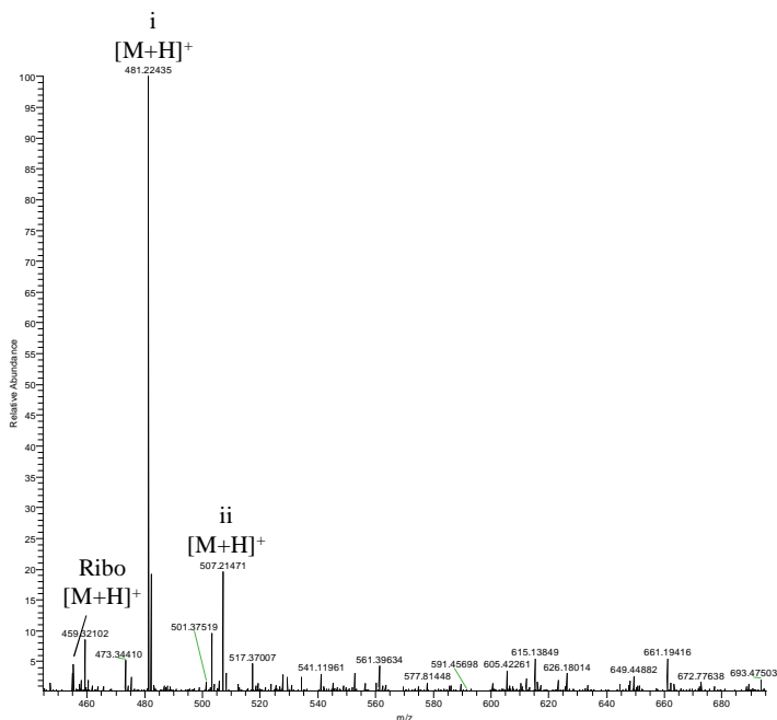
Figure 5.14: ESI-MS spectrum of reaction mixture of ribostamycin (Ribo) with 16 equiv. diazo-transfer reagent 7.HCl after incubation for 18 hours at room (i-ii = number of introduced azide groups).
