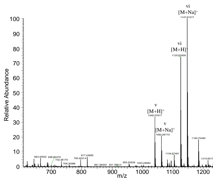
Figure 4.21: ESI-MS spectrum after transformation of neomycin B with 30 equiv. isopropyl isocyanate 9b in absence of APG ( v-vi = number of introduced urea groups).
