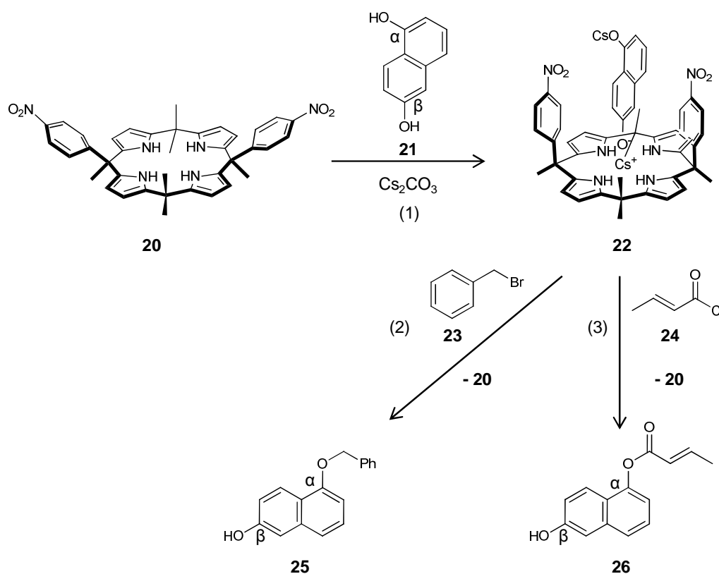
Scheme 1.6: Regioselective modification of hydroxy naphthol 21 employing calix[4]pyrrol 20 as SPG: Selective complexation (1), regioselective alkylation (2) and regioselective acylation (3). 18
