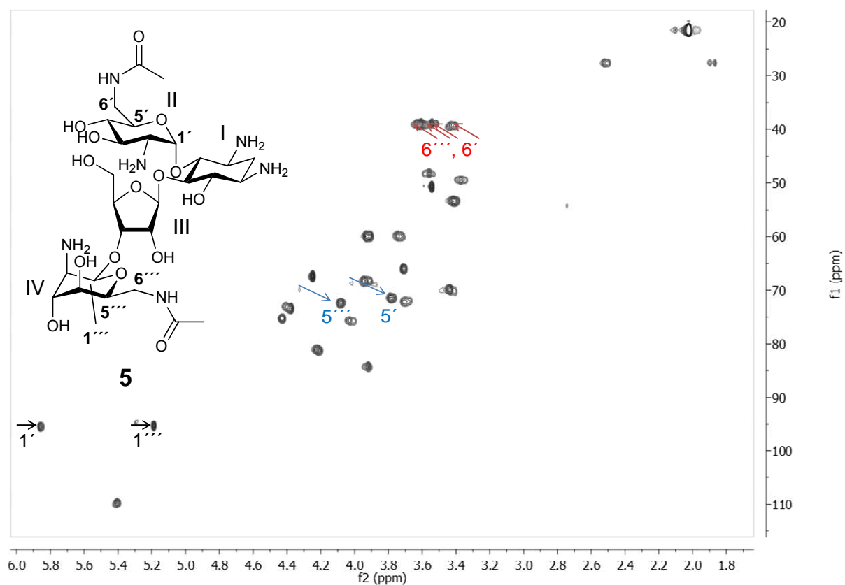
Figure 3.9: HSQC (500 MHz, \text{D}_2\text{O} ) spectrum of 6',6'''- N -diacetyl neomycin B x 4 HFBA 5 . Arrows indicate the chemical shift of J(\text{C}6\text{-H}) - (red), J(\text{C}5\text{-H}) - (blue) and J(\text{C}1\text{-H}) coupling (black) of ring II and IV.
