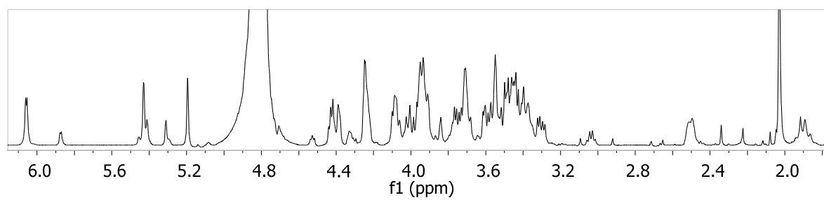
Figure 4.11a: ^1\text{H-NMR} (500 MHz, \text{D}_2\text{O} ) spectrum of 6'''- N -acetyl neomycin B x 5 HFBA 10 .
