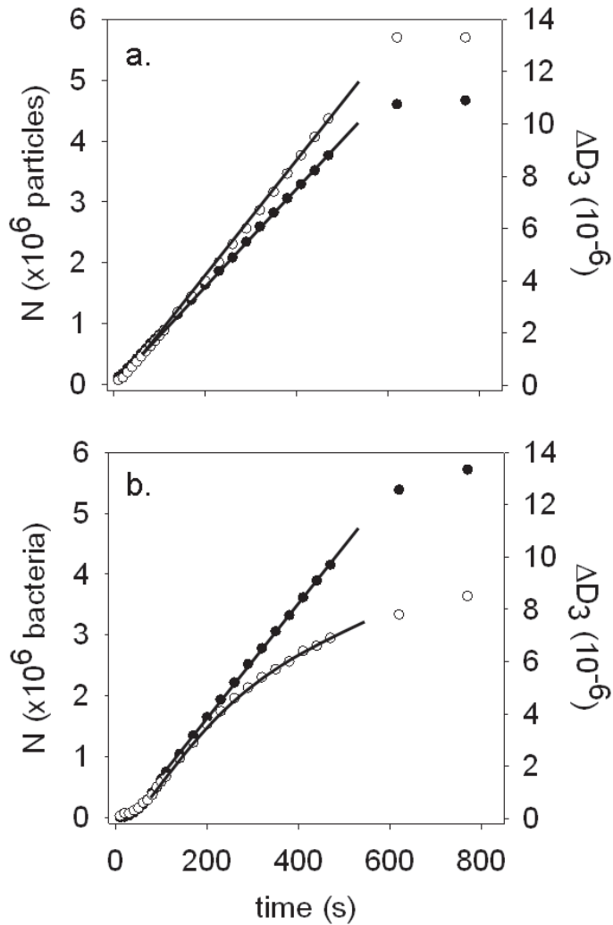
Figure 1. Increase in the number of adhering particles and bacteria N ( \bullet , left axis) and measured dissipation shift \Delta D ( \circ , right axis) as a function of time, for silica particles (panel a) and S. salivarius HB7 (panel b). A linear increase in the number of adhering silica particles is accompanied by a linear increase in measured dissipation shift, whereas a linear increase in bacterial numbers is accompanied by a non-linear change in dissipation, indicating a time-dependent rearrangement in the bacterium-substratum interfacial region.
