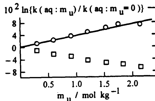
Figure 3. Dependence of \ln(k/k^0) for hydrolysis of p-methoxyphenyl dichloroethanoate in aqueous solution as a function of molality of added urea: experimental points (O) and calculated dependence (full line) using G(\text{CONH} \leftrightarrow \text{OH}^\ddagger) = -20 \text{ J kg}^{-1} . The points ( \square ) are calculated with G(\text{CONH} \leftrightarrow \text{OH}^\ddagger) set to zero, the trend being a consequence of added urea on chemical potential of water in urea (aq).
