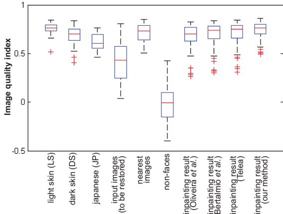
Figure 9: Structural image quality for the input images, face database, and result images.
