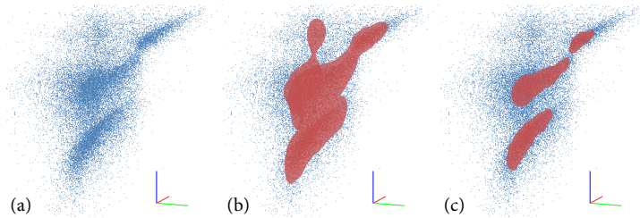
Figure 4.10: CloudLasso being applied to a 3D scatter plot; data from a subset of the milliMillennium dataset [De Lucia and Blaizot, 2007] (showing the dimensions virial radius, R-I color, and low X-ray luminosity); (a) original 3D scatter plot, (b) initial CloudLasso selection, (c) after interactive threshold adjustment.
