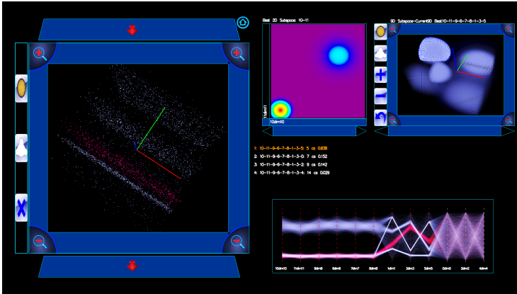
Figure 5.1: Interface of the proposed system. Left half: window I_1 for a 3D spatial plot. Right half: (top left) window I_2 for a 2D scatter plot / density plot; (top right): window I_3 for a 3D scatter plot / density plot; (bottom): window I_4 for a parallel coordinate plot of parametric space.
