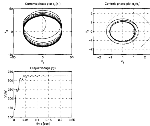
Fig. 6: Response of the system under the proposed controller
