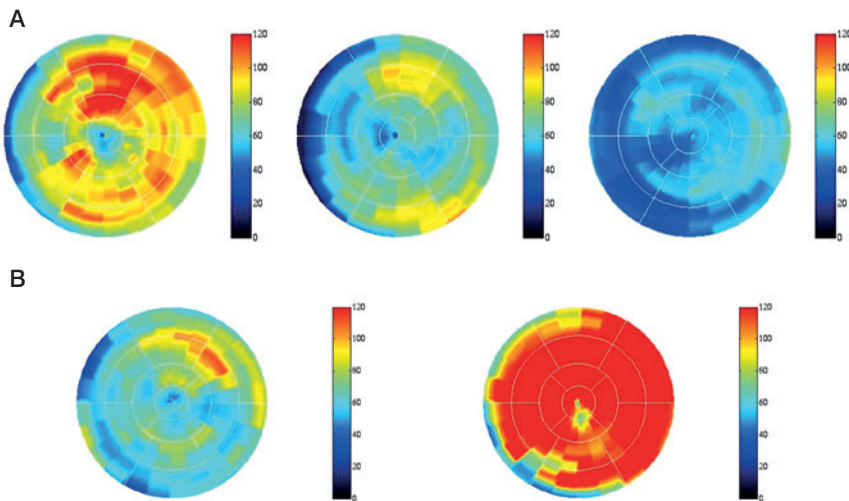
Figure 1 Polarmap reconstruction of [^{13}\text{N}]\text{ammonia} PET scans.
