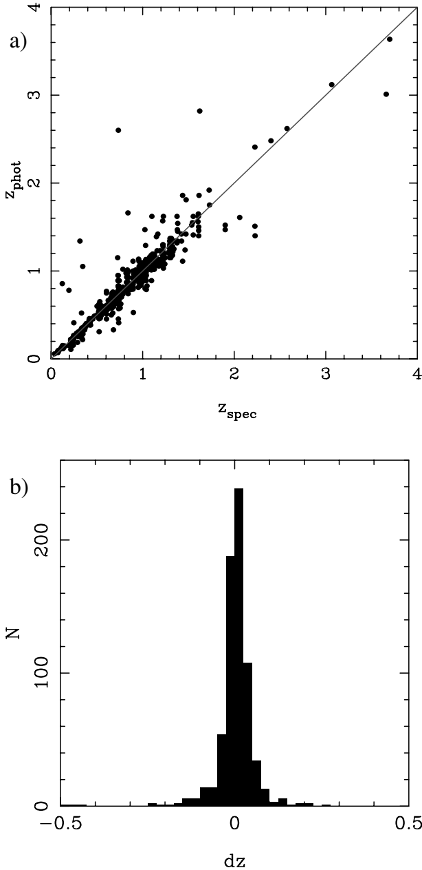
Figure 2. (a) Photometric versus spectroscopic redshifts for K_s < 21.5 galaxies in the GOODS/CDFS. (b) Distribution of relative errors. The median of this distribution is dz = (z_{\text{spec}} - z_{\text{phot}})/(1 + z_{\text{spec}}) = 0.01 and the rms \sigma = 0.03 .
