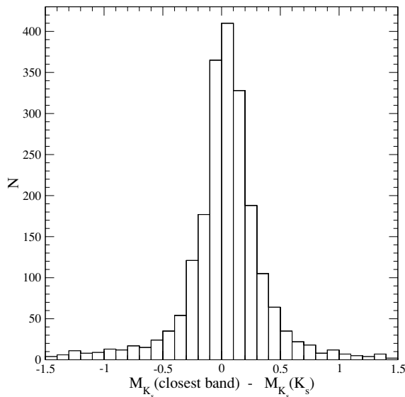
Figure 5. The distribution of the differences between the rest-frame absolute K_s -band magnitudes M_{K_s} obtained from the closest available rest-frame band and the ones obtained extrapolating from the observed K_s magnitudes in all cases. The distribution is centred at M_{K_s}(\text{closest}) - M_{K_s}(K_s) = 0.04 and the rms \sigma = 0.24 .
