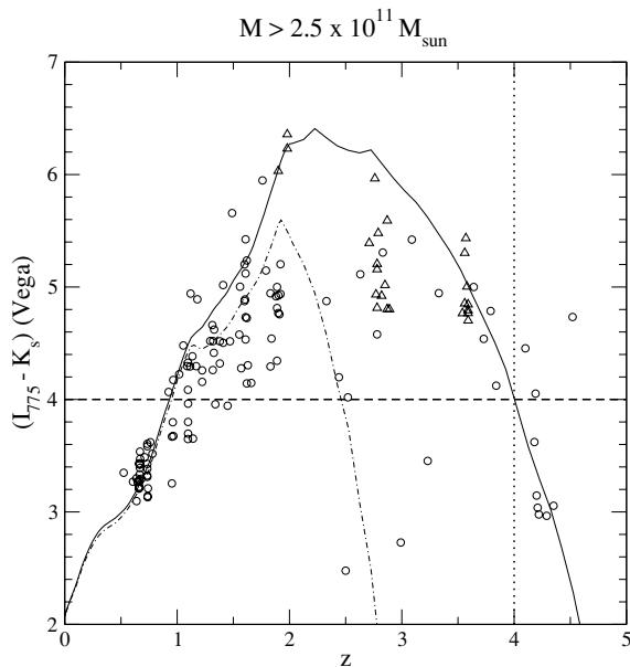
Figure 8. The observed (I_{775} - K_s) colours versus redshift for galaxies with estimated stellar mass M > 2.5 \times 10^{11} M_{\odot} . The symbols are the same as in Fig. 7. The solid and dotted–dashed lines show the modelled evolution of the (I_{775} - K_s) colours for galaxies formed in an instantaneous burst at redshift z_f = 5 and 3, respectively, both with no dust and passive evolution thereafter.
