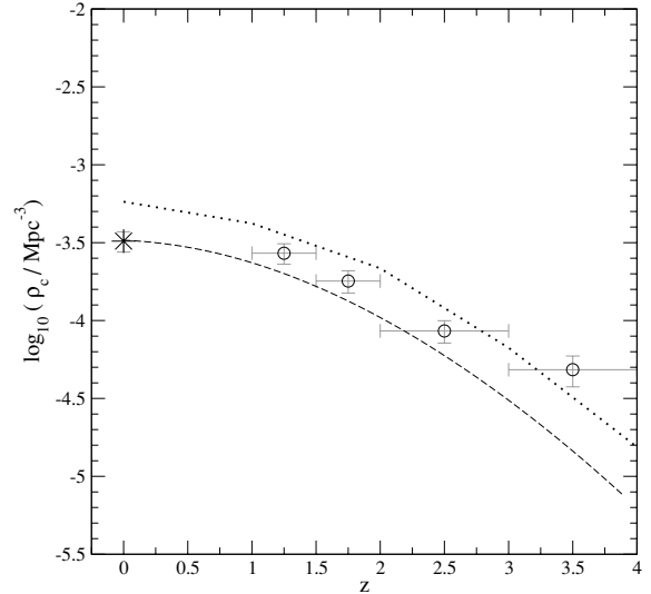
Figure 10. The comoving number density of galaxies with stellar mass M > 1 \times 10^{11} M_{\odot} (considering the IMF of Chabrier 2003). The symbols are the same as in Fig. 9.
