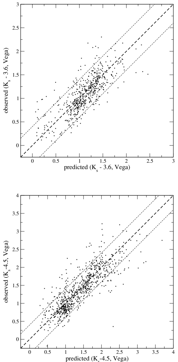
Figure 12. The observed versus predicted ( K_s - [3.6 \mu\text{m}] ) and ( K_s - [4.5 \mu\text{m}] ) colours (upper and lower panels, respectively) for the K_s < 21.5 (Vega) galaxies in the restricted area of the GOODS/CDFS studied by Caputi et al. (2005a). The dashed lines indicate the region of consistency, taking into account the error bars on the observed colours.
