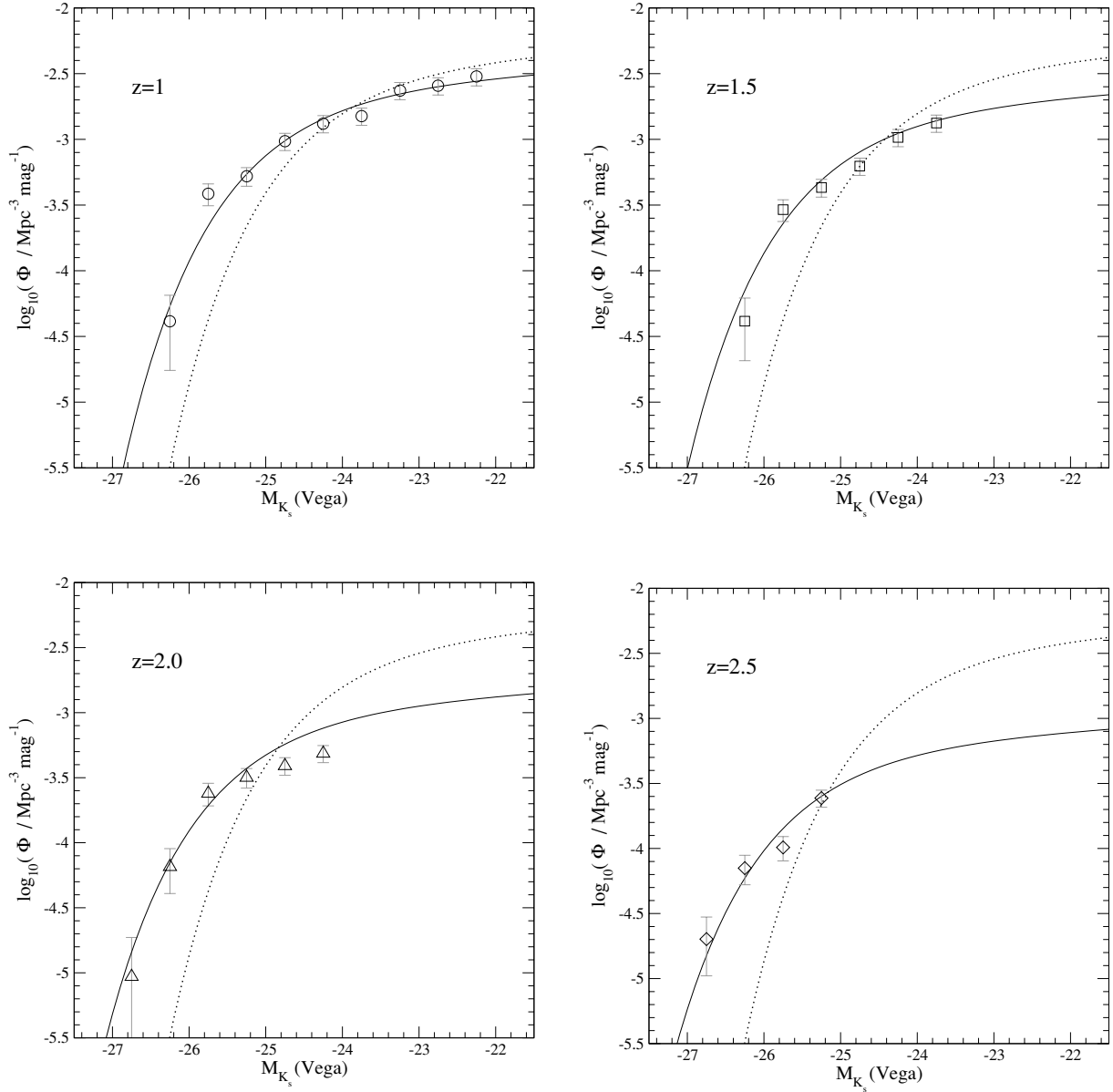
Figure 6. The rest-frame K_s -band luminosity function at redshifts ( z ) = 1.0, 1.5, 2.0 and 2.5 (circles, squares, up-triangles and diamonds, respectively). The empty symbols correspond to the LF computed with the 1/V_{\max} method. Only values above the luminosity-completeness limits of each redshift bin are shown. The solid lines show the resulting LF obtained through the ML analysis. For a comparison, we show in each panel the local K -band LF measured from 2MASS data by Kochanek et al. (2001; dotted lines).
