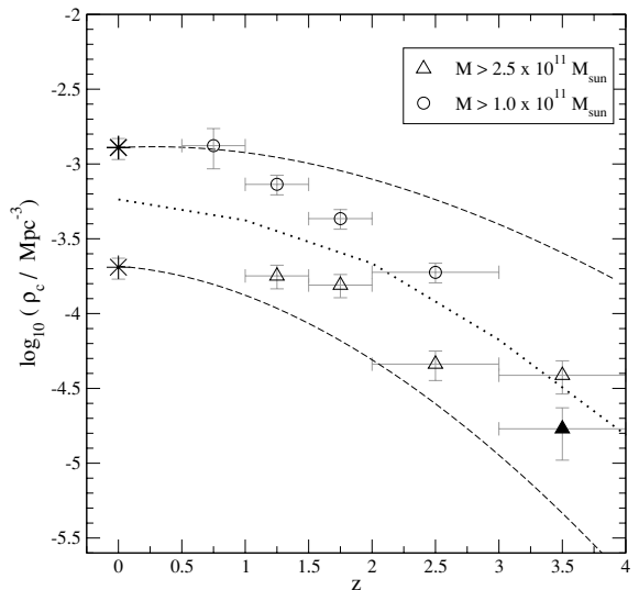
Figure 9. The comoving number density of galaxies with stellar mass M > 1 \times 10^{11} M_{\odot} (circles) and M > 2.5 \times 10^{11} M_{\odot} (triangles) (Salpeter 1955 IMF, restricted to M = (0.1-100) M_{\odot} ). The filled triangle at z = 3.5 denotes the recomputed number density of M > 2.5 \times 10^{11} M_{\odot} galaxies after correcting for the effects of large-scale structure in the corresponding redshift bin. The star-like symbols indicate the density values for the same mass thresholds at z = 0 , obtained integrating the local stellar mass function (Cole et al. 2001; Bell et al. 2003). The dashed lines show the evolution of the number density of haloes with total mass M > 2 \times 10^{12} M_{\odot} and M > 1 \times 10^{13} M_{\odot} (upper and lower curves, respectively), as obtained from Lambda cold dark matter ( \lambda CDM) models of structure formation (with a code kindly provided by Will Percival). The dotted line corresponds to the predicted number density of galaxies with mass M > 1 \times 10^{11} M_{\odot} obtained with SPH simulations (Nagamine et al. 2005).
