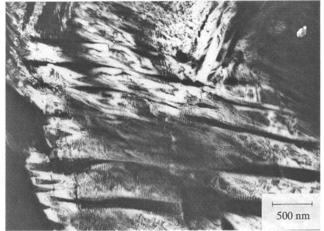
FIG. 9. Dark-field TEM image of Cr 3 O 4 on duplex SAF 2205 showing larger twins than in Cr 3 O 4 on Fe 22 wt. % Cr (Fig. 5).
