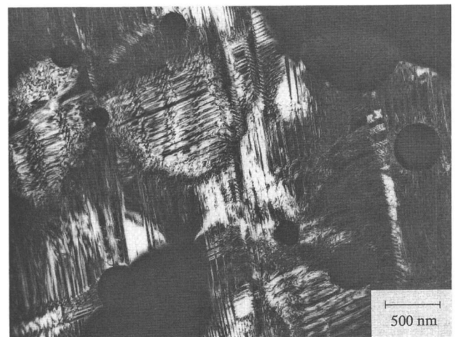
FIG. 5. Dark-field TEM image of \text{Cr}_3\text{O}_4 coating on Fe 22 wt.% Cr showing a very fine twinned structure.
