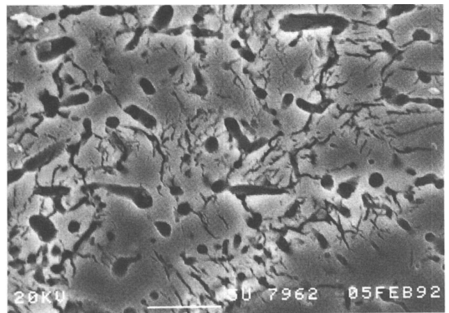
FIG. 4. Etched X-section of \text{Cr}_3\text{O}_4 coating on Fe 22 wt.% Cr showing microcracks. Holes are due to etching of \text{FeCr} particles. Etched in modified Groesbeck.
