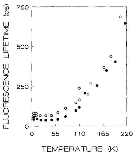
FIG. 5. Fluorescence decay time as a function of temperature for the blue (●) and red (○) excitonic origins of PIC-Br.
