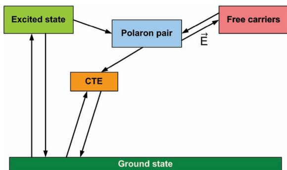
Figure 7. Schematic representation of the excitation in the BHJ under study. For simplicity only the excited state of the polymer is indicated, triplet levels are also omitted.
