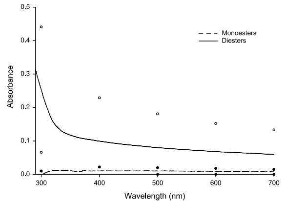
Fig. 1. Absorption spectra of mono- (dashed line) and diester (solid line) preen waxes. Six samples of monoesters were analysed and four samples of diesters. Dots indicate 95% confidence intervals at 100 nm increments for monoesters (black dots) and diesters (white dots).
