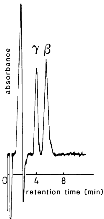
Figure 2. Representative chromatogram of 100 \mu\text{l} of plasma spiked with 20 \mu\text{g} of \beta -cyclodextrin and 110 \mu\text{g} of \gamma -cyclodextrin (method B).
