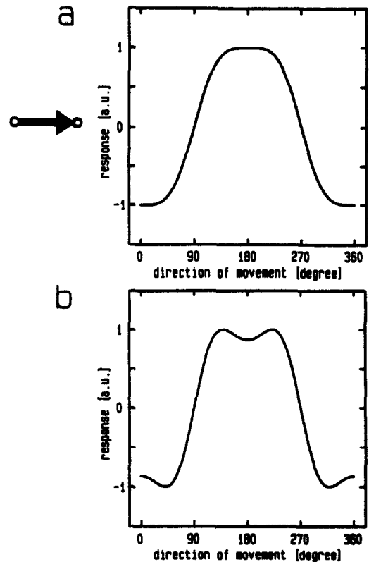
Fig. 5. Directional tuning curves of a multiplicative movement detector (Reichardt correlator), in (a) for the spatial wavelength optimally exciting the detector ( \lambda = 4\Delta\phi ), and in (b) for a slightly smaller, but still quite effective wavelength ( \lambda = 3\Delta\phi ). The curves are given by equation (10) (see text).
