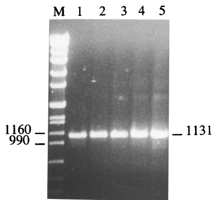
FIG. 7. PCR products formed on chromosomal DNA of lactococcal strains MG1363 (lane 1), IL1403 (lane 2), 18-16s (lane 3), AM1 (lane 4), and HP (lane 5). The primers used were PALA-4 and PALA14 (Fig. 4). Lane M, molecular weight markers (bacteriophage Spp1 DNA cut with EcoRI ), sizes of which (in base pairs) are indicated on the left and right.
