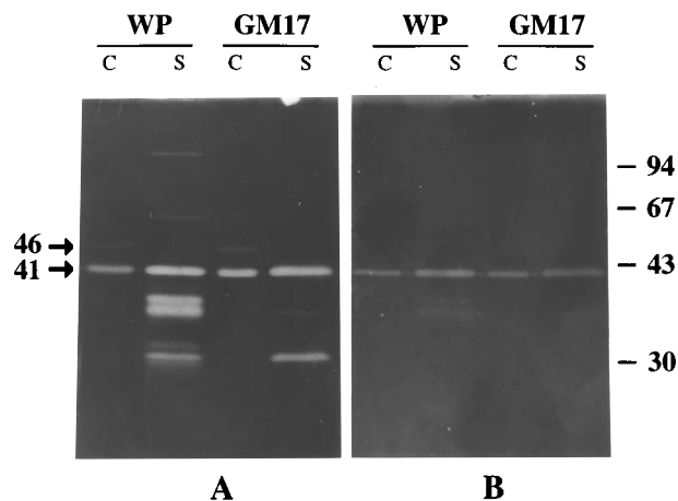
FIG. 1. Cell wall hydrolase activity of L. lactis MG1363 in renaturing SDS-12.5% PAGE. (A) Gel containing 0.2% (wt/vol) M. lysodeikticus autoclaved cells; (B) gel containing 0.2% (wt/vol) cell walls from L. lactis MG1363. Lanes: WP and GM17, fractions of cultures grown in whey-based medium and GM17, respectively; C, cell extract; S, supernatant fraction. The amount of sample loaded was equalized according to the optical density of the cultures. Molecular masses (in kilodaltons) of standard proteins are shown on the right, and the sizes (in kilodaltons) of two lytic bands discussed in the text are indicated on the left.
