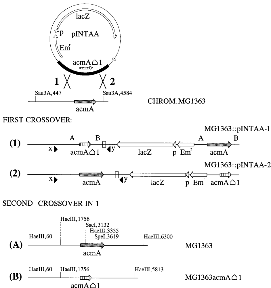
FIG. 8. Schematic representation of construction of chromosomal acmAΔ1 mutant of L. lactis with pINTAA. Closed bar, insert of pAL09 in pORI280; acmAΔ1 , deletion derivative of acmA ; Emr r , erythromycin resistance gene; lacZ , β-galactosidase gene of E. coli expressed under control of lactococcal promoter P 32 (p); open square, origin of replication of lactococcal plasmid pWV01; 1 and 2, possible sites for the first crossover; x and y, primers PALA-19 and BK05AL, respectively, used to distinguish between two types of Campbell integrants (labelled 1 and 2); A and B, possible regions for a second crossover and their products (labelled A and B). A number of relevant restriction enzyme sites are also shown.
