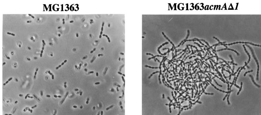
FIG. 10. Light microscopic view of L. lactis MG1363 (left) and MG1363 acmA \Delta 1 (right). Both strains were grown overnight in GM17. Magnification, \times 1,000 .
