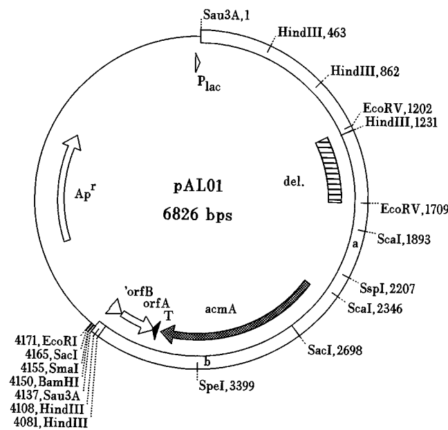
FIG. 3. Map of pAL01. The 4,137-bp Sau3A DNA fragment of the chromosome of L. lactis MG1363 is indicated by the open bar. pAL01 includes acmA , ORFA, and ORFB. T, putative terminator; P_{lac} , lac promoter and its direction of transcription (open arrowhead); del., EcoRV deletion made to construct pAL02; Ap^r , ampicillin resistance gene. The HindIII-SacI fragments used to construct pAL04 and pAL03 are indicated by a and b, respectively. The genetic analysis of the 2,206-bp Sau3A-SspI fragment will be presented elsewhere (3a).
