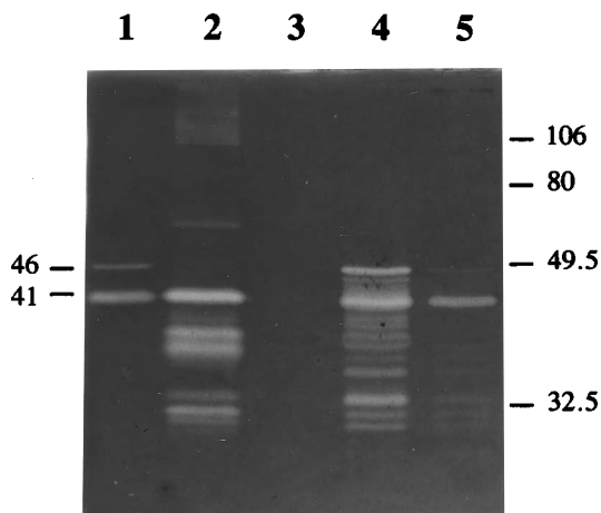
FIG. 2. Cell wall hydrolase activity in E. coli NM522 transformants by rearing SDS-12.5% PAGE. The gel contained 0.2% (wt/vol) M. lysodeikticus autoclaved cells. Lanes: 1 and 2, cell extract and supernatant of L. lactis MG1363 grown in whey-based medium, respectively; 3, cell extract of E. coli NM522; 4 and 5, cell extracts of two independent E. coli NM522 transformants producing a halo on TY plates containing M. lysodeikticus autoclaved cells. Molecular masses (in kilodaltons) of standard proteins are shown on the right. Two lytic bands corresponding to sizes of 41 and 46 kDa are indicated on the left.
