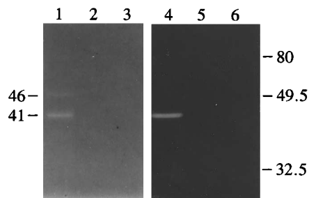
FIG. 9. AcmA activity in L. lactis MG1363 (lanes 1 and 4) and deletion mutants MG1363 acmA \Delta 1-a (lanes 2 and 5) and acmA \Delta 1-b (lanes 3 and 6) by renaturing SDS-12.5% PAGE. The gel contained 0.2% (wt/vol) M. lysodeikticus autoclaved cells. Cell extracts (lanes 1 to 3) and supernatant fractions (lanes 4 to 6) after growth in GM17 were applied. The amount of sample was equalized according to the optical density of the cultures. Molecular masses (in kilodaltons) of standard proteins and of mature AcmA (46) or its secreted form (41) are shown on the right and left, respectively.
