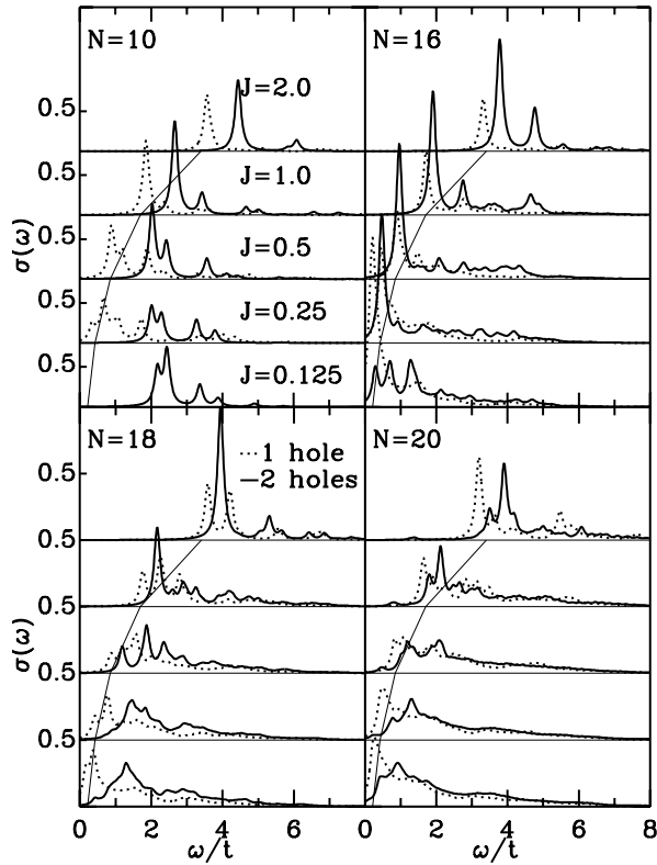
Figure 7.1: Exact diagonalization result of the optical conductivity spectrum of one or two holes doped into a cluster of size N for the t - J model, reproduced from Eder, Wróbel and Ohta [242]. The relevant parameter set for the cuprates is J=0.25t . The thin solid line denotes \omega = 1.7J .
