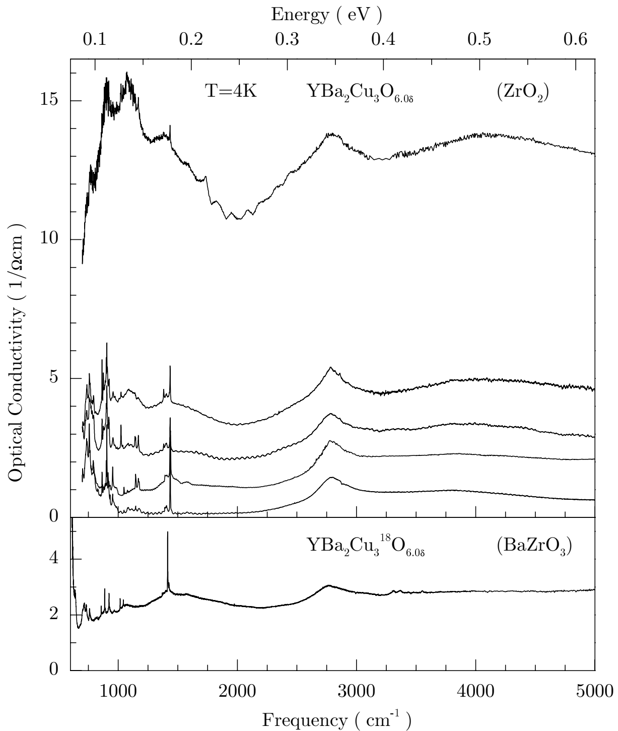
Figure 7.8: Mid-infrared \sigma(\omega) spectra of YBa_2Cu_3O_x in the low doping regime x < 6.1 at 4 \text{ K} . Note the very low values of \sigma(\omega) . Top panel: samples grown in \text{ZrO}_2 crucibles; bottom panel: oxygen isotope substituted sample of YBa_2Cu_3^{18}O_6 grown in a \text{BaZrO}_3 crucible.
