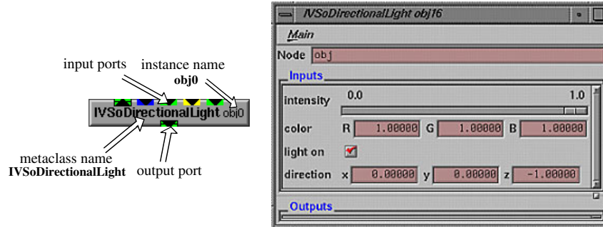
Figure 3: Left: Visual icon for a metaclass. Several graphical signs encode the ports' C++ types, by value/by reference transfer, and other attributes. Right: automatically built GUI for the metaclass
