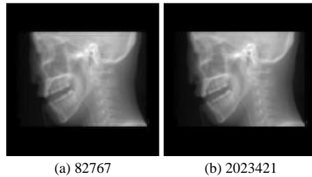
Figure 5. Comparison of a partial reconstruction using only 4% of the coefficients (a) and the full reconstruction (b).
