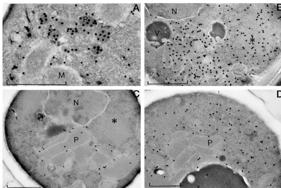
FIG. 3. Immunocytochemical demonstration of peroxisomal proteins in glycerol-grown \Delta pex14::P_{AOX}PEX5^{2c} cells (A) or methanol-induced \Delta pex14::P_{AOX}PEX5^{mc} (B–D). By using \alpha -AO antisera the small peroxisomes present in glycerol-grown \Delta pex14::P_{AOX}PEX5^{2c} cells are labeled. Part of the AO protein is, however, mislocated in the cytosol (A). A similar labeling pattern is observed using \alpha -DHAS antisera in methanol-induced \Delta pex14::P_{AOX}PEX5^{mc} (B) (*, AO aggregate). The peroxisomal membrane protein Pex3p is properly inserted into the membrane of these peroxisomes as was evident upon labeling using \alpha -Pex3p antibodies (C) (*, AO aggregate). Unexpectedly, CAT protein was confined to the cytosol and absent in the peroxisomes present in \Delta pex14::P_{AOX}PEX5^{mc} cells ( \alpha -CAT; D) glutaraldehyde-fixation. The abbreviations used are as follows: M, mitochondrion; N, nucleus; P, peroxisome; V, vacuole. The marker represents 0.5 \mu m.
