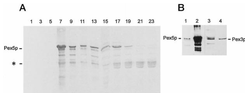
FIG. 8. A , Western blot showing the distribution of Pex5p in the odd fractions of a sucrose gradient prepared from homogenized methanol-induced \Delta pex14::P_{AOX}PEX5^{mc} cells (compare Fig. 4C) using \alpha -Pex5p antibodies. A prominent band is observed at the position where WT peroxisomes are located (fraction 7). The soluble portion of Pex5p protein has most likely been subject to proteolytic degradation, as is suggested by the strong protein bands at 30 kDa in fractions 17–23 (indicated by *). B , Western blots prepared from purified peroxisomes, using \alpha -Pex5p (lanes 1 and 2) and \alpha -Pex3p (lanes 3 and 4) antibodies. Compared with WT peroxisomes (lane 1), peroxisomes from \Delta pex14::P_{AOX}PEX5^{mc} cells contain enhanced amounts of Pex5p (lane 2). The amount of Pex3p is somewhat higher than in WT organelles (lane 3) compared with peroxisomes from \Delta pex14::P_{AOX}PEX5^{mc} cells (lane 4). Peroxisomes were purified by sucrose density centrifugation. Equal amounts of protein were loaded per lane.
