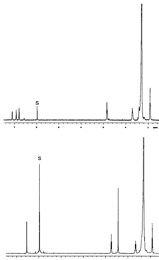
Figure 1. ^1\text{H} NMR spectra ( \text{C}_2\text{D}_2\text{Cl}_4 , 95°C) of (a, top) \text{H}(\text{CH}_2\text{CH}_2)_n\text{-}2\text{-C}_4\text{H}_3\text{S} and (b, bottom) \text{H}(\text{CH}_2\text{CH}_2)_n\text{-}2\text{-(5-Me-C}_4\text{H}_2\text{S)} , prepared with catalyst \mathbf{4b} in neat thiophene and 2-methylthiophene respectively.
