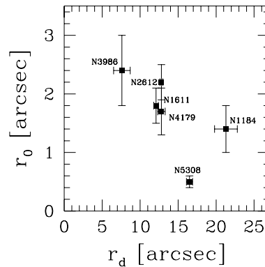
Figure 14. Plot of the estimates of photometric disc scale length r_d vs. the estimates of the parameter r_0 for the gravitational potential.
