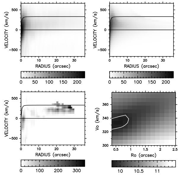
Figure 7. Same as in Fig. 2 for NGC 5308
