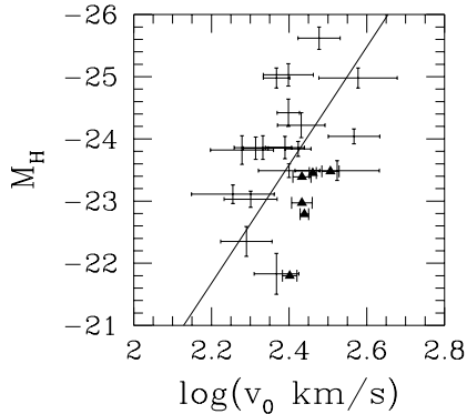
Figure 16. Estimated absolute H -band magnitude versus \log(v_0/\text{km/s}) for the sample of S0 galaxies in Neistein et al. (1999), and those in this analysis (filled triangles). The line shows the H -band Tully-Fisher relation for later-type spirals from Pierce & Tully (1992).
