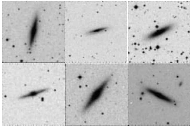
Figure 1. Images from Digitized Sky Survey for the sample of S0 galaxies. From Left to Right, Top to Bottom: NGC1184, NGC1611, NGC2612, NGC3896, NGC4179 and NGC5308.
