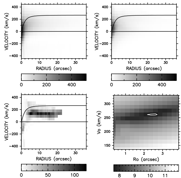
Figure 4. Same as in Fig. 2 for NGC 2612
