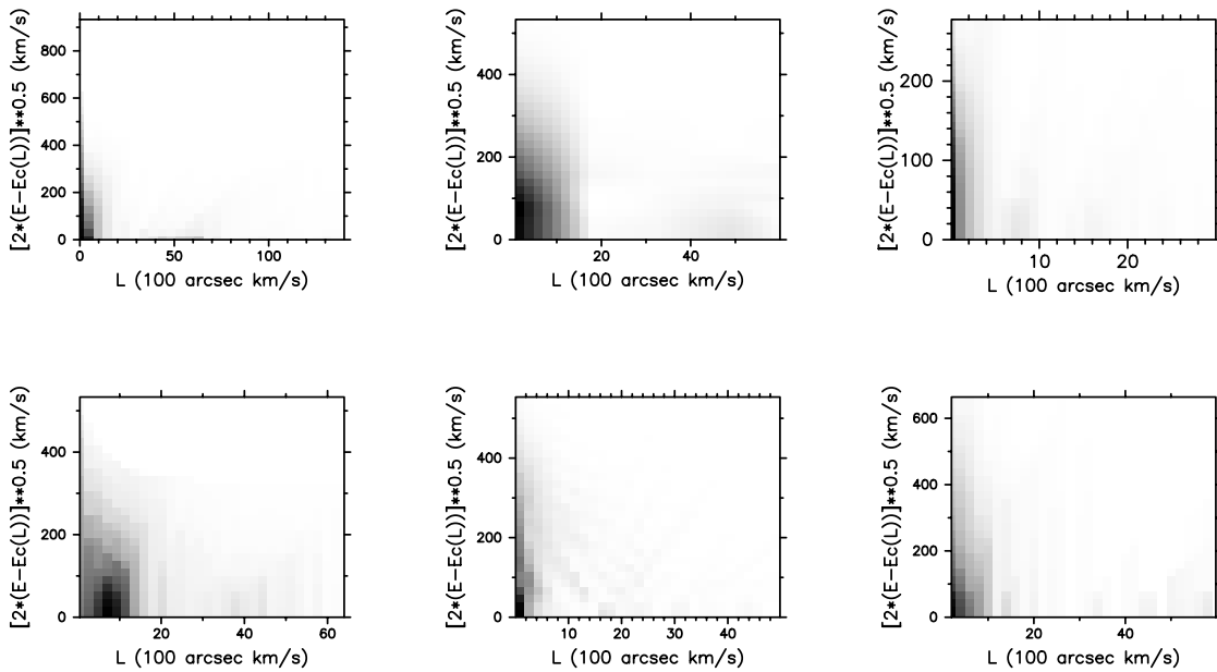
Figure 8. The disc distribution functions for the galaxies as derived iteratively from their line-of-sight kinematics using the best-fit gravitational potentials.
