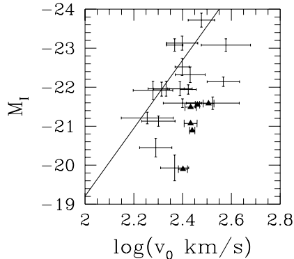
Figure 15. Absolute I -band magnitude versus \log(v_0/\text{km/s}) for the sample of S0 galaxies in Neistein et al. (1999), and those in this analysis (filled triangles). The line shows the I -band Tully-Fisher relation for later-type spirals from Pierce & Tully (1992).
