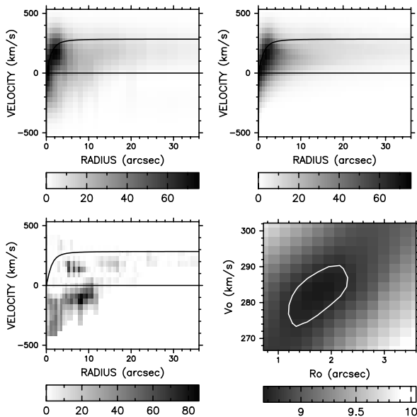
Figure 10. Same as in Fig. 2 for NGC 3986, using data on the "right" side of the galaxy.
