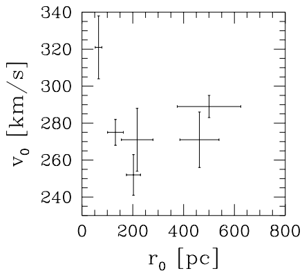
Figure 13. Plot of the estimates of the maximum circular velocity v_0 vs. the estimates of the parameter r_0 .
