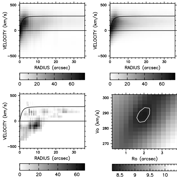
Figure 5. Same as in Fig. 2 for NGC 3986
