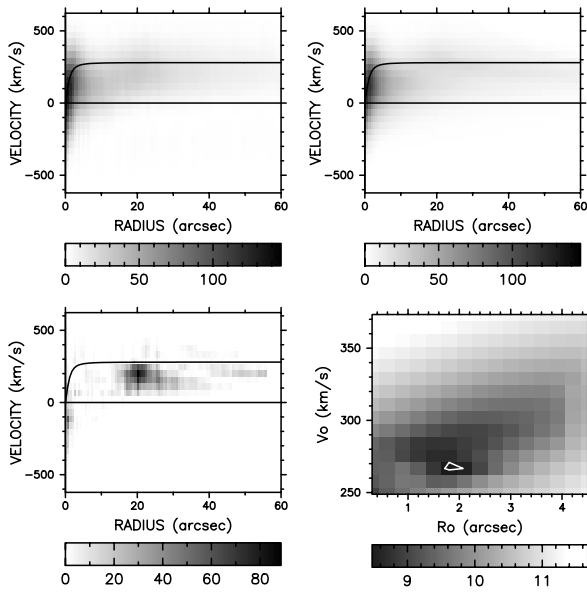
Figure 2. Top left: The line-of-sight velocity distribution as a function of projected radius along the major axis of NGC 1184. Top right: the corresponding quantities for the best-fit dynamical model. Bottom left: plot of [(\text{data-model})/\sigma]^2 , showing where the major \chi^2 residuals arise. Bottom right: \ln(\chi^2) as a function of the adopted parameters for the gravitational potential, (r_0, v_0) ; the solid contour shows where \ln(\chi^2) = \ln(1.1 \times \chi_{min}^2) .
