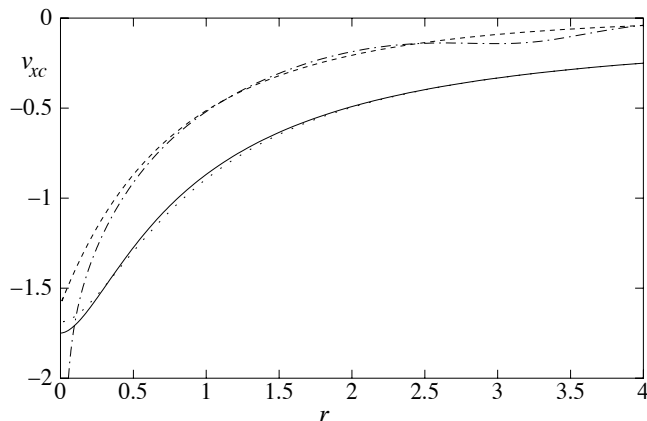
Fig. 1. The exchange-correlation potential for helium: exact (solid), exact exchange-only approximation (dotted), local density approximation (dashed) and the PW91 generalized gradient approximation (dashed-dotted).
