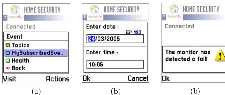
Figure 7: Viewing the topic tree (a), registering for an event (b), and receiving a notification (c).
