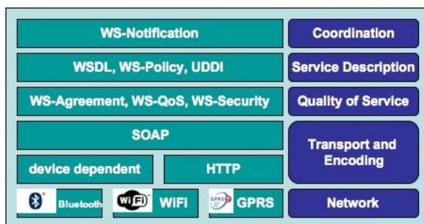
Figure 6: The Web Service stack implementation for Domotics.
