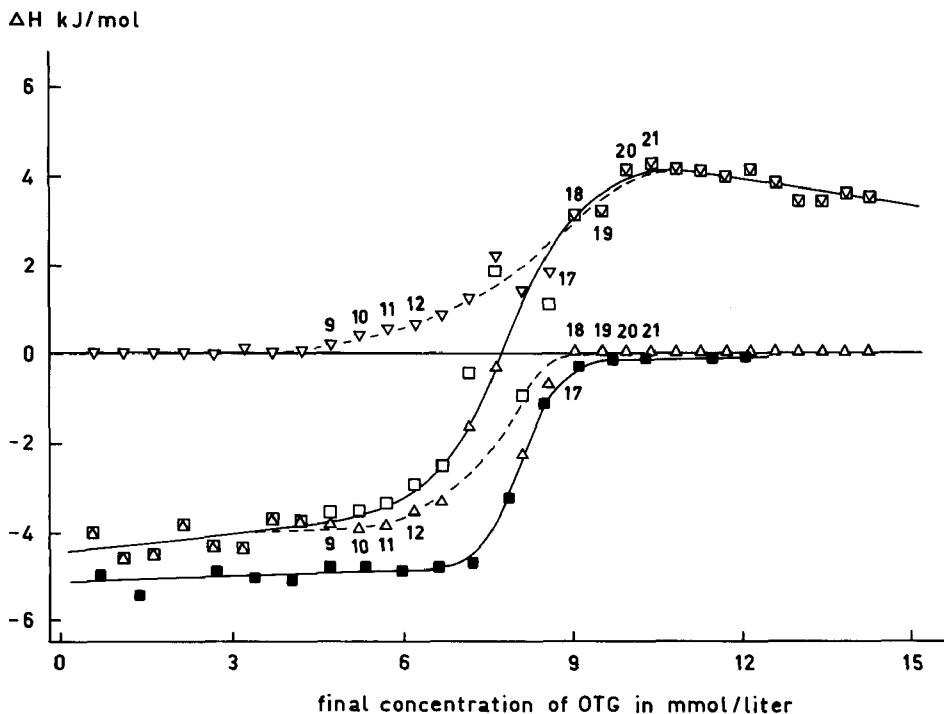
Figure 2.4 Enthalpy of dilution as a function of the final OTG concentration in water or in an aqueous solution of PPO at 25 °C.; (■) in water, cmc = 8.05 \times 10^{-3} ; in PPO solutions: ( \Delta ) exothermic effect, ( \nabla ) endothermic effect, ( \square ) summation of exothermic and endothermic effect. The numbers (9-12; 17-21) correspond with the titration steps indicated in Figure 2.3.
